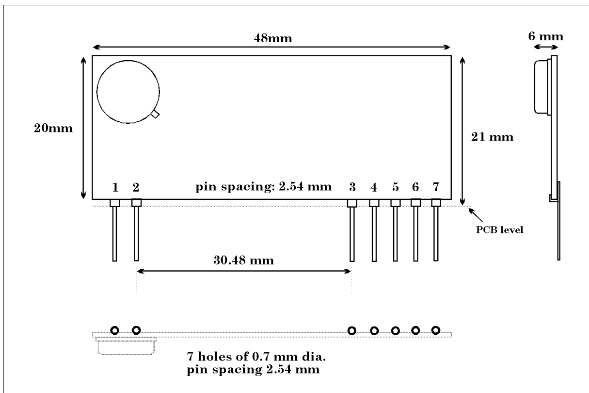
figure 3: Mechanical Dimensions:
