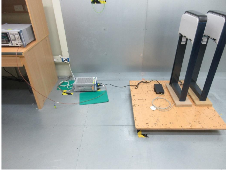
Photograph 7: Test Setup for Mains Conducted Emissions (Back View)
