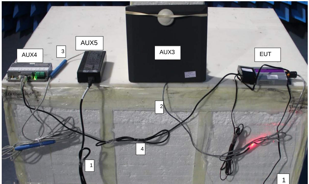
Figure 1b: Test Setup Photos – EUT in combination with Antenna
