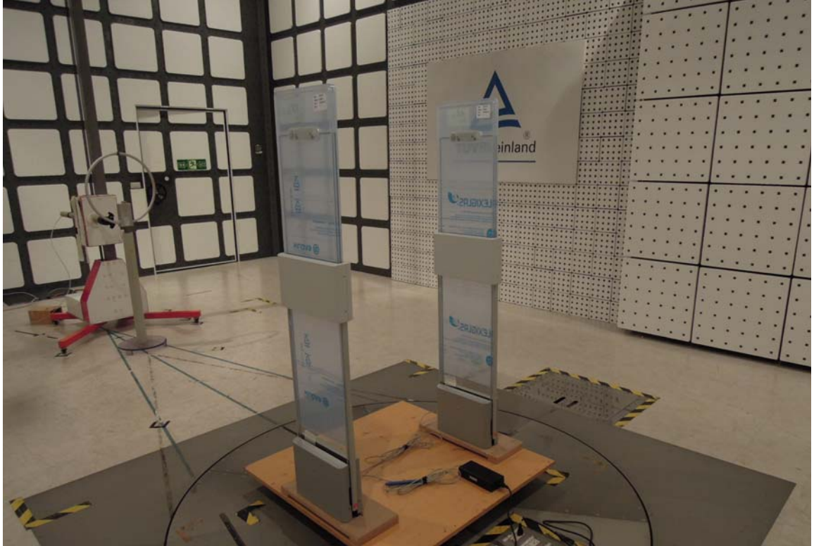
Photograph 2: Set-up for Radiated Emissions (Back View 1)
