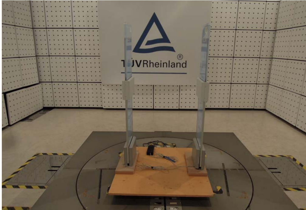
Photograph 1: Set-up for Radiated Emissions (Front View)
