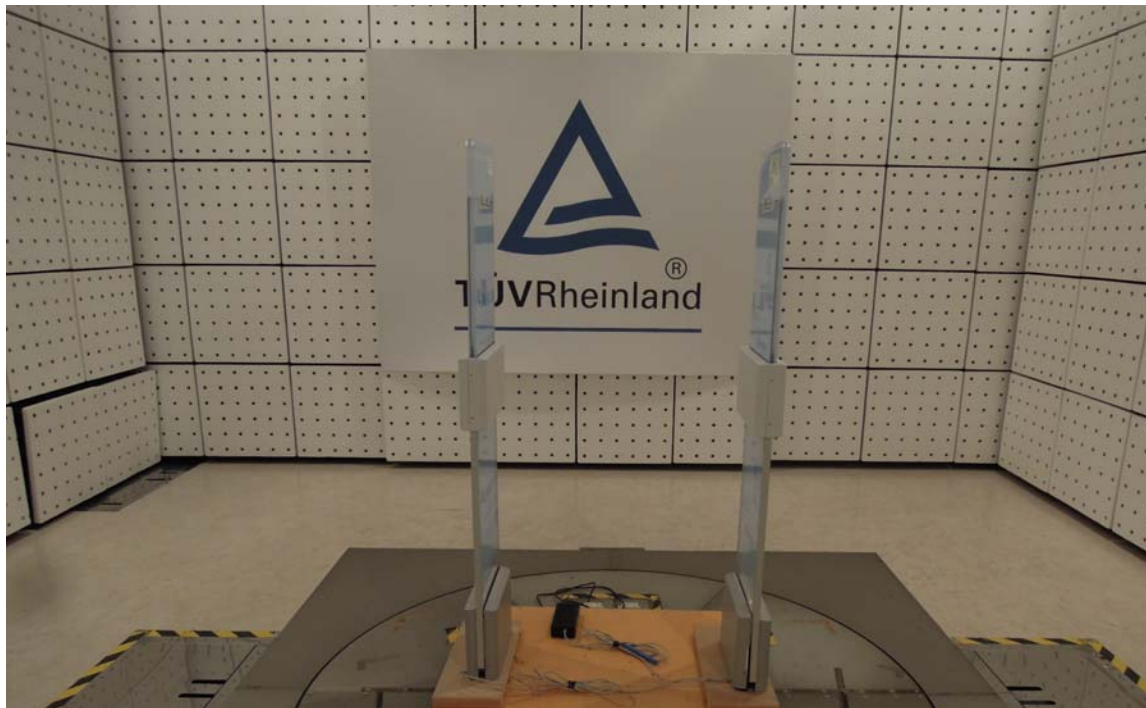
Photograph 1: Set-up for Radiated Emissions TX (Front View)
