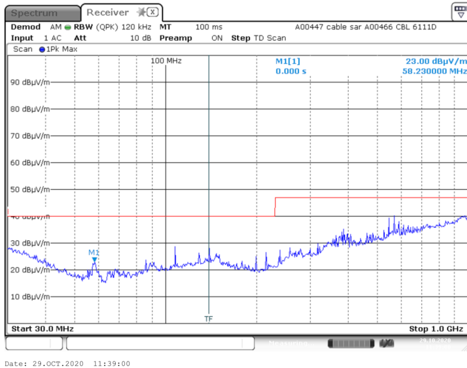
Plot 1a: radiated emissions of the EUT(vertical), Antenna vertical, in the range 30 – 1000 MHz (pre-scan -peak values shown).
