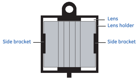
Figure 15. Mask installation
