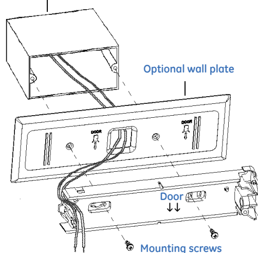
Figure 3. Mounting and wiring access
