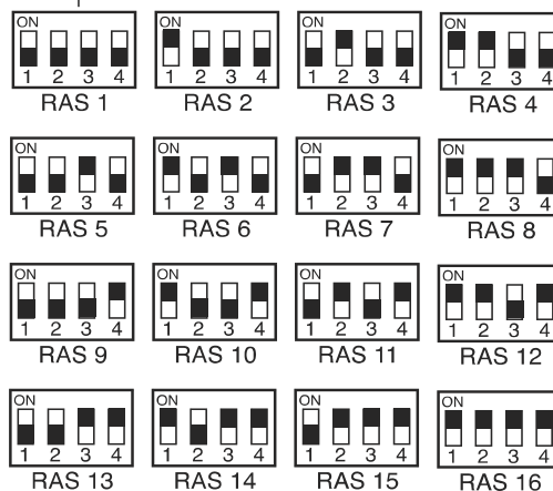
Figure 3. RAS Address DIP Switch Settings
