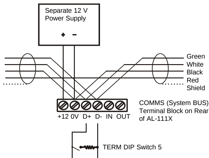
Figure 4. Connections for Powering the RAS from a Separate Power Supply
