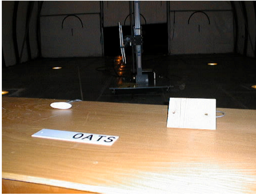
Figure 6.19 - Radiated Emissions, Open Area Test Site (NX1700E)
