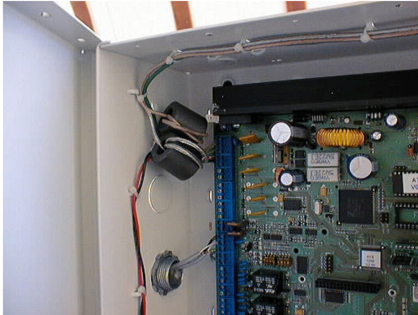
Figure 6.21 - Modifications To The Device (AL-1251)
