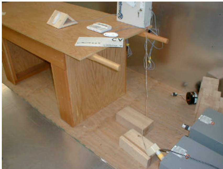
Figure 6.11 - Conducted Voltage Emissions Measurement Configuration (NX-1700E)
