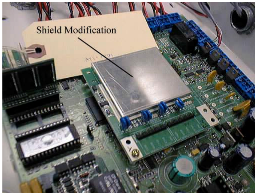
Figure 6.25 - Modifications To The Device (AL-1801)
