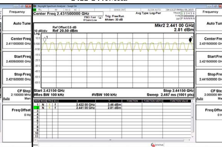
2422-2441MHz
