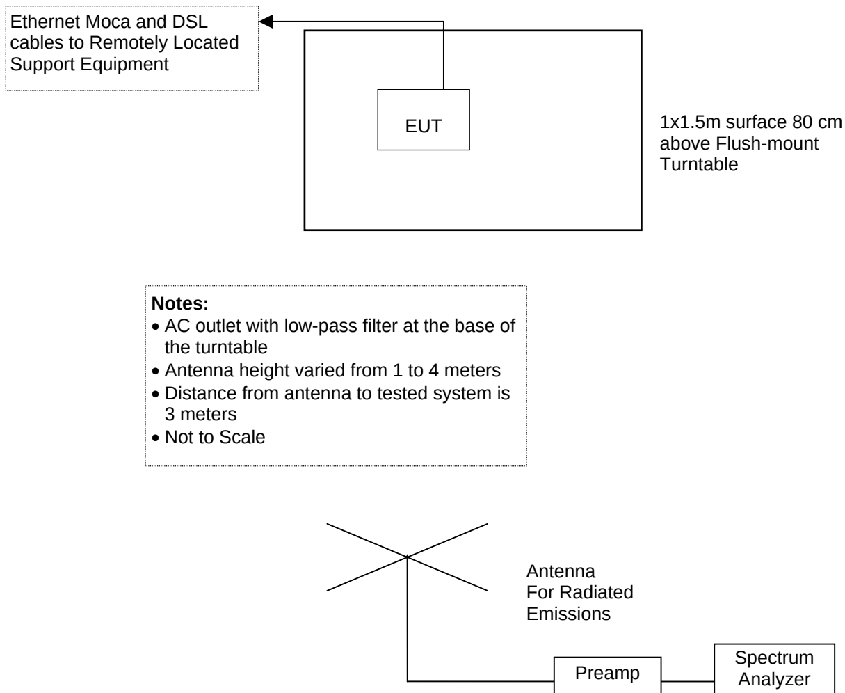
Figure 2. Drawing of Radiated Emissions Setup
