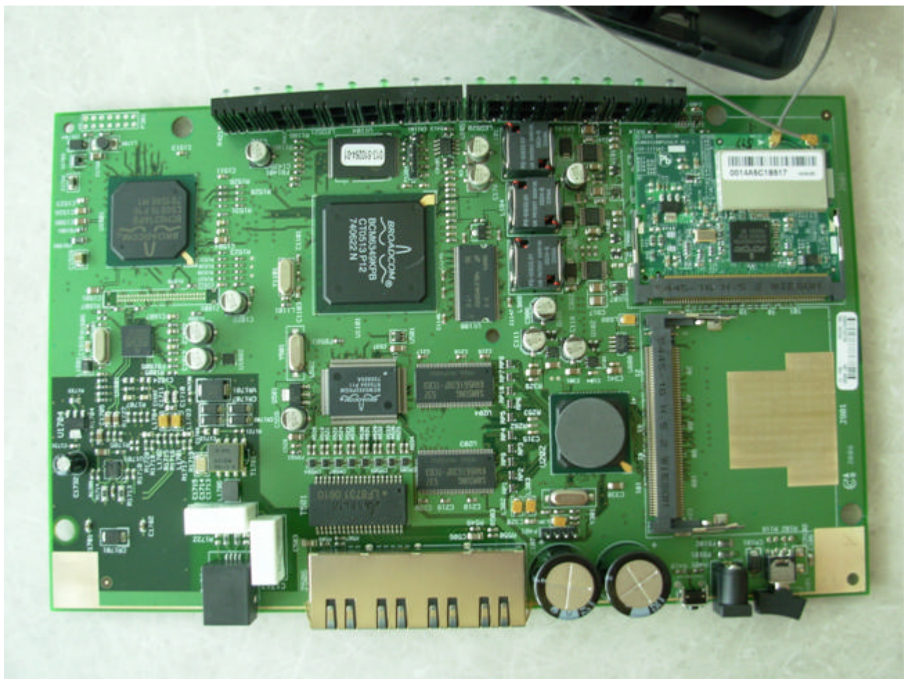
Photograph of Main Processor Board:
