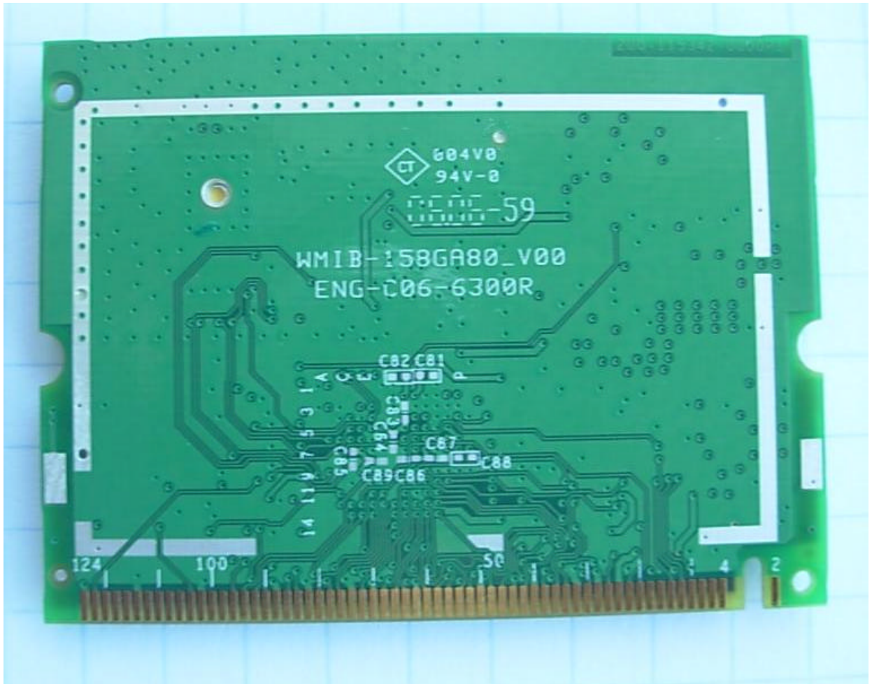
Rear of WiFi Board
