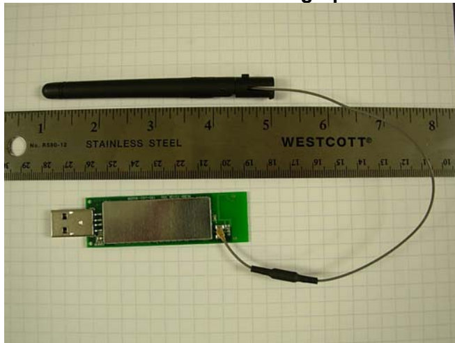
Photographs of RF PCB and 2.4 GHz Antenna
