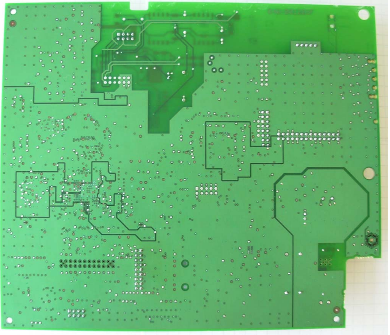
Photograph of Telephony LCD PC board: Bottom
