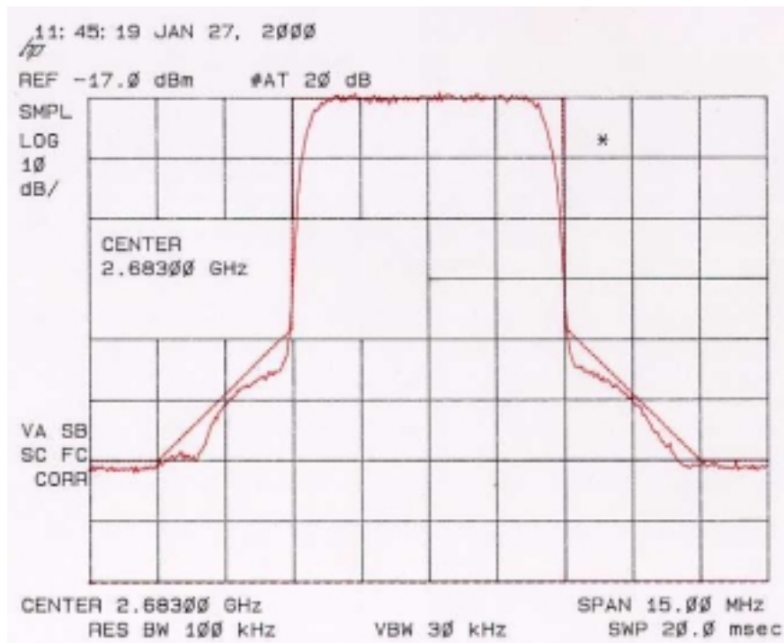
PLOT 6: Occupied bandwidth of the 256 QAM transmitter.
