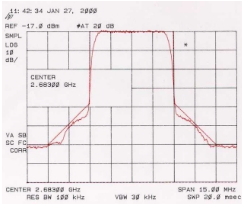
PLOT 5: Occupied bandwidth of the 64 QAM transmitter.
