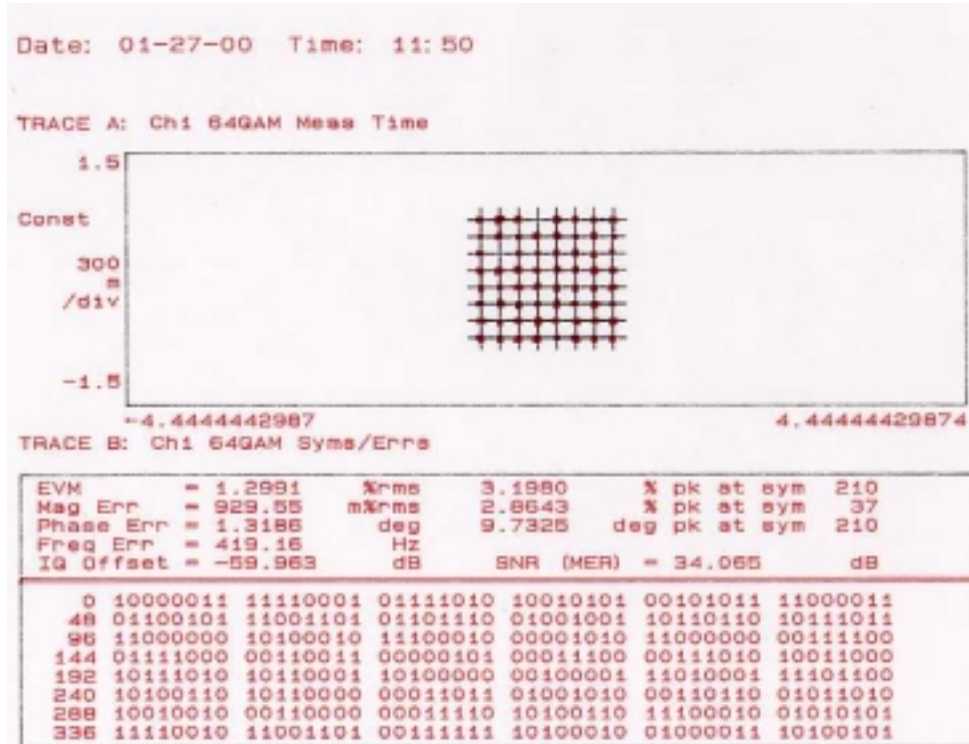
PLOT 1: Demodulation performance of the 64 QAM transmitter.
