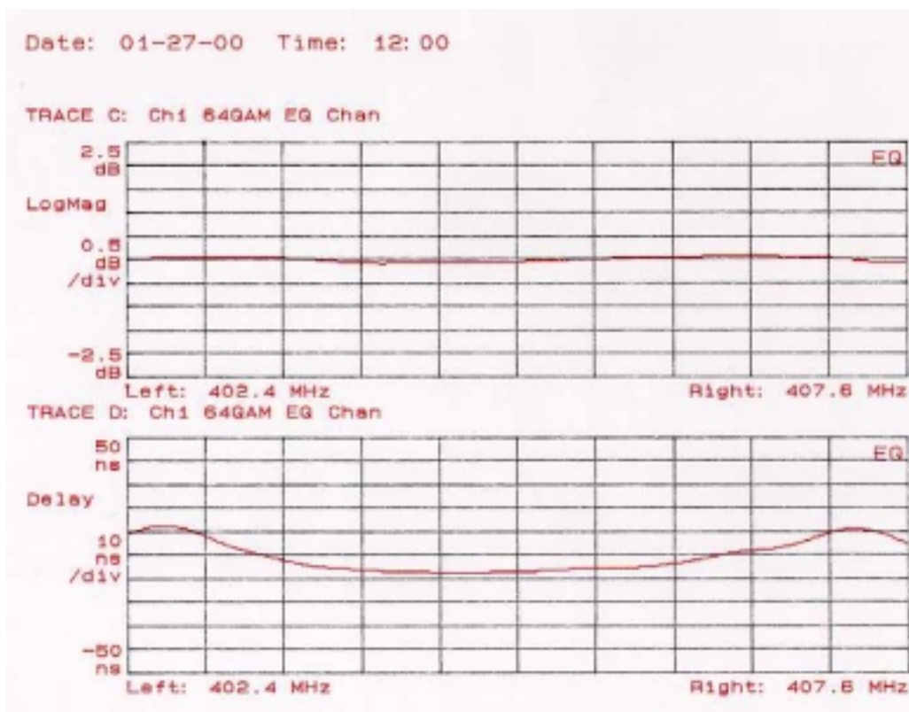
PLOT 3: Frequency response and group delay of the 64 QAM transmitter.
