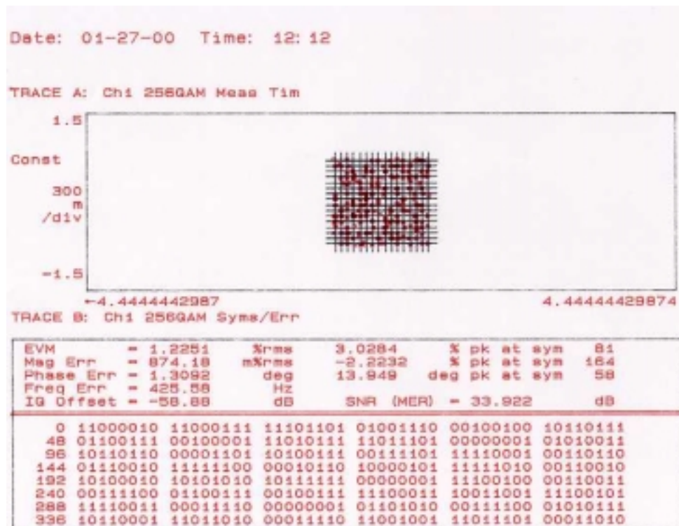
PLOT 2: Demodulation performance of the 256 QAM transmitter.
