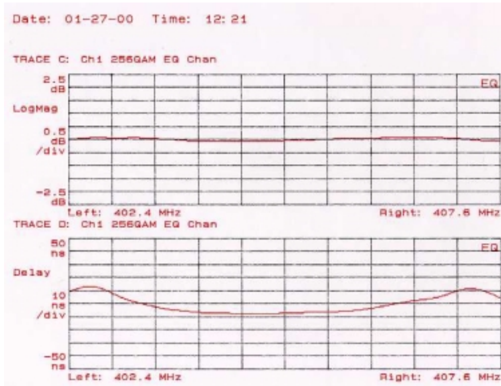
PLOT 4: Frequency response and group delay of the 256 QAM transmitter.
