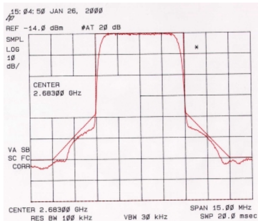
PLOT 6: Occupied bandwidth of the 256 QAM transmitter.
