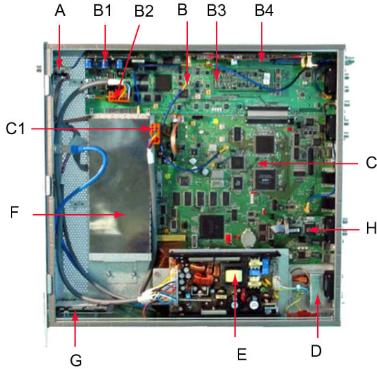
Figure 1 Exciter (top view)
