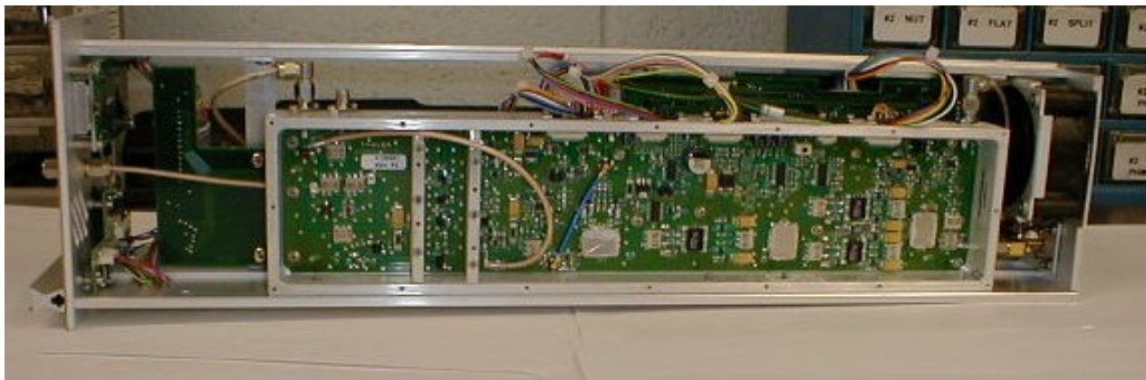
Figure 5 Upconverter plug-in
