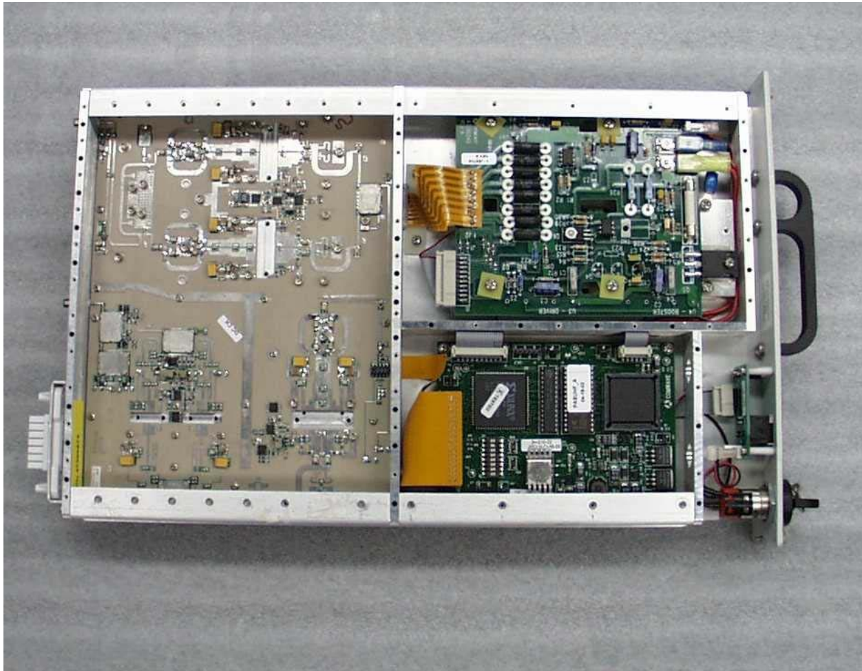
Figure 6 Power amp plug-in
