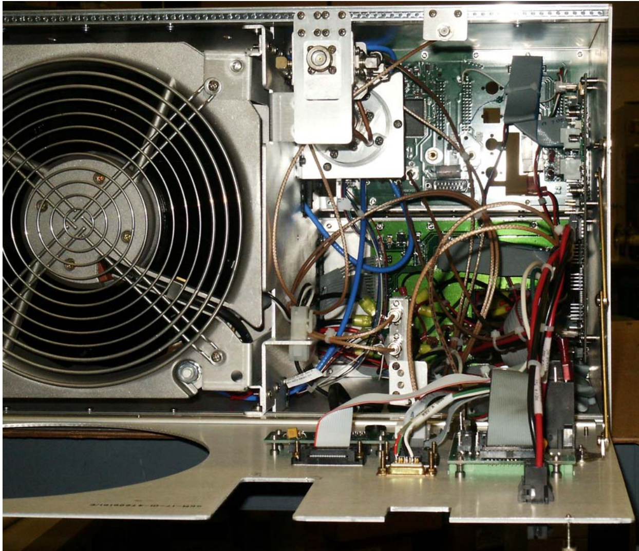
Figure 3: Affinity upconverter amplifier chassis (rear view)
