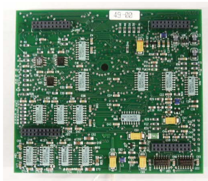
Figure 2 47266058 PCB Bottom Side View
