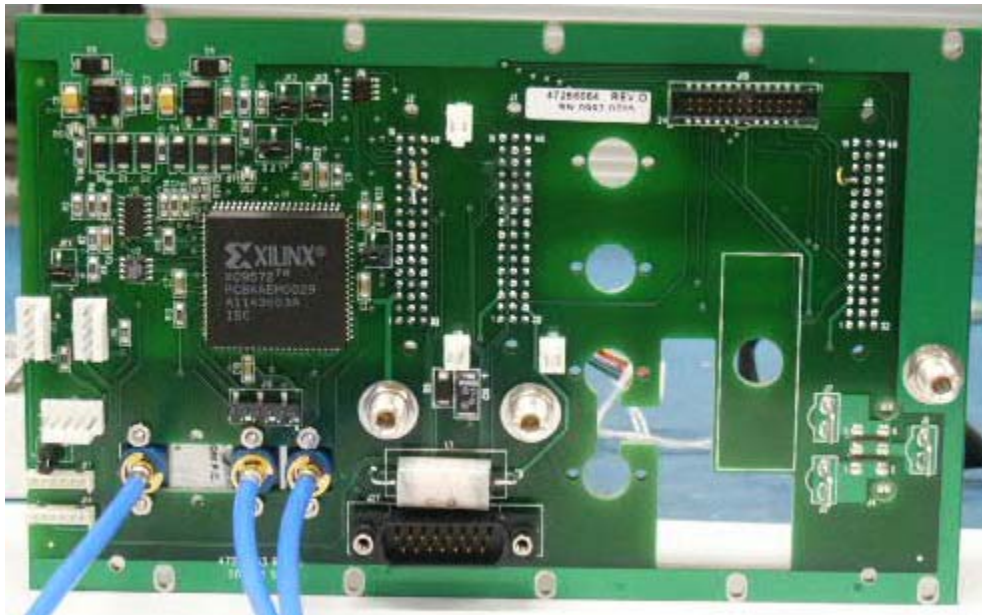
Figure 12 47266064 PCB Bottom Side View
