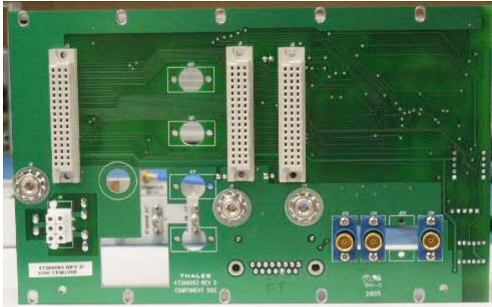
Figure 11 47266064 PCB Top Side View
