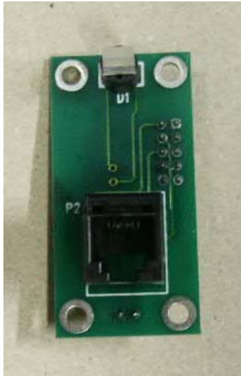
Figure 17 47267249 PCB Top Side View
