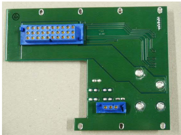
Figure 10 47266165 PCB Bottom Side View
