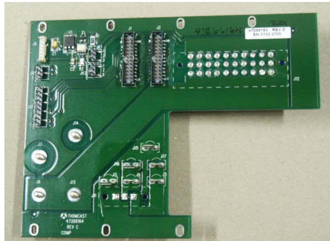
Figure 9 47266165 PCB Top Side View
