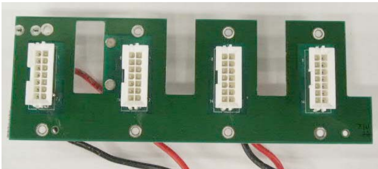
Figure 28 47266294 PCB Bottom Side View
