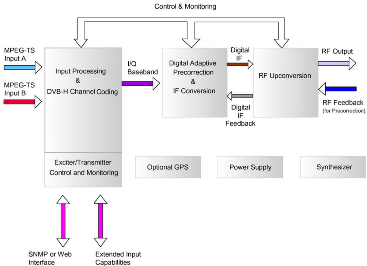
Thales DVB-H Digital Exciter Block Diagram
