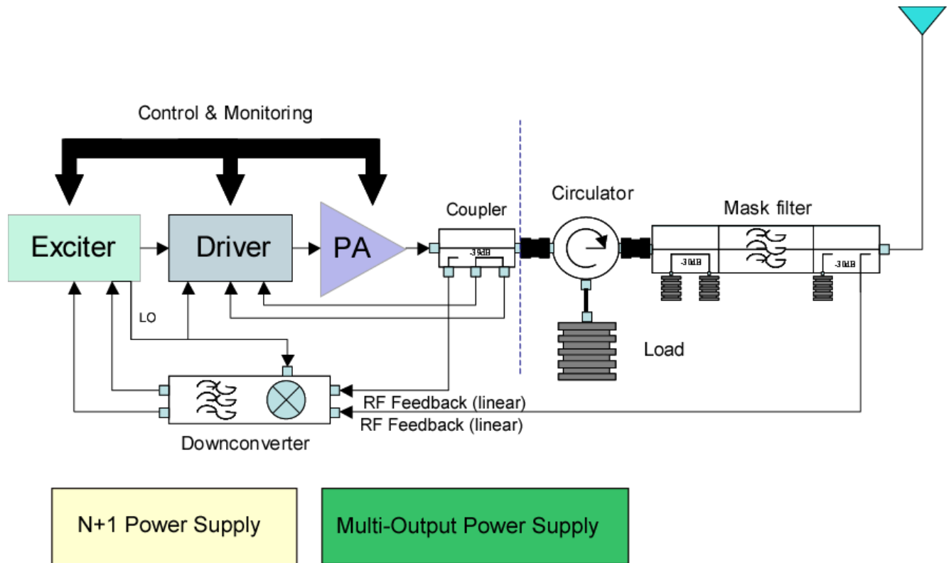
Simplified Transmitter Block Diagram
