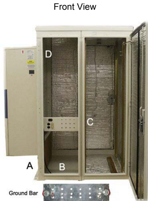
Earth Grounding Scheme
