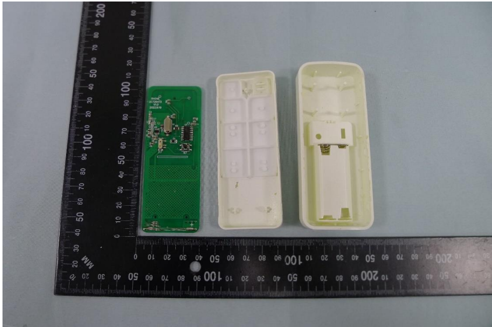
(6) EUT Photo (UC7264T3A)
