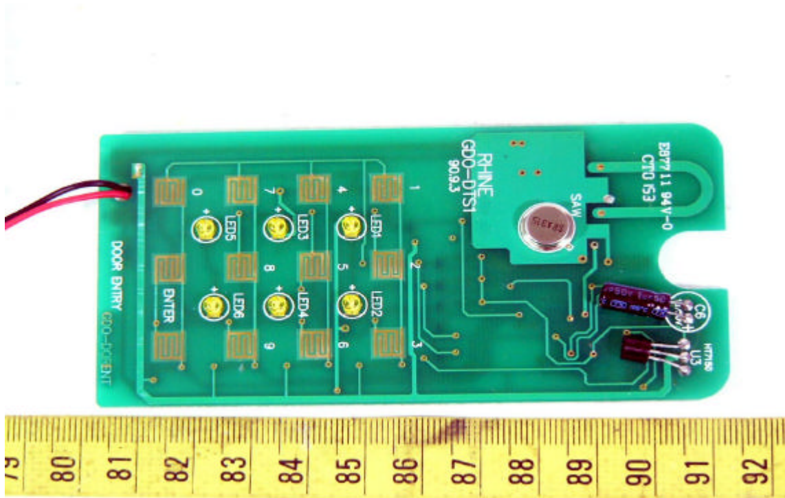
Component View of Main PCB
