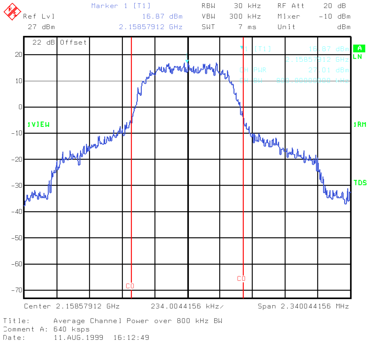
Plot 13 – QPSK Modulation, 640 ksps
