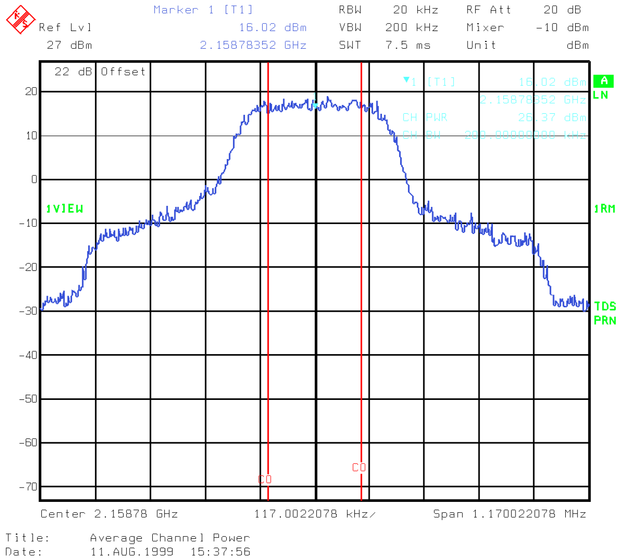
Plot 7 - QPSK modulation, 320 kbps
