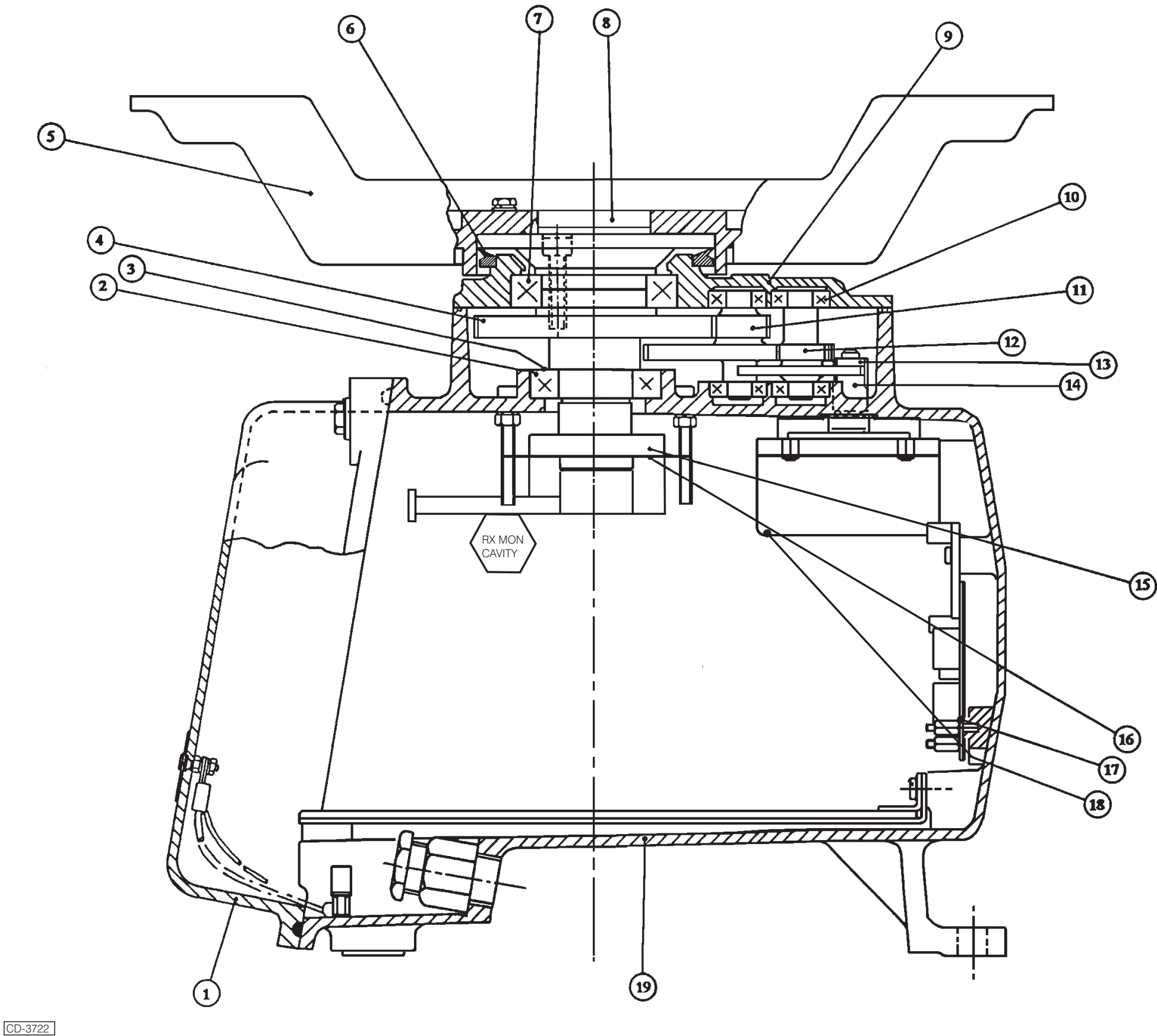
Turning Mechanism: Main Assemblies
