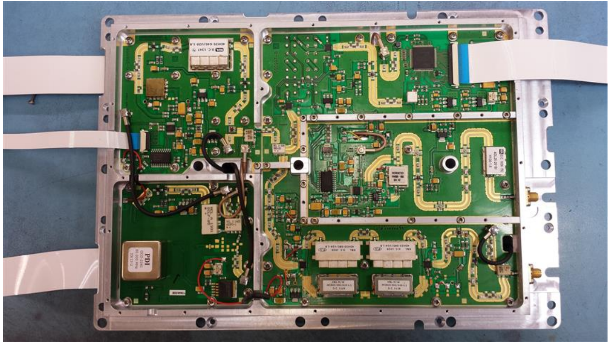
DTX-A213 UPCONVERTER
