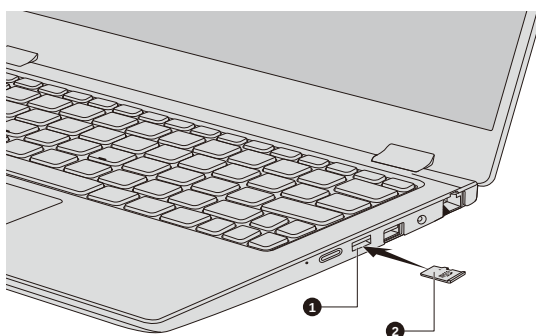
Figure 4-4 Inserting memory media
