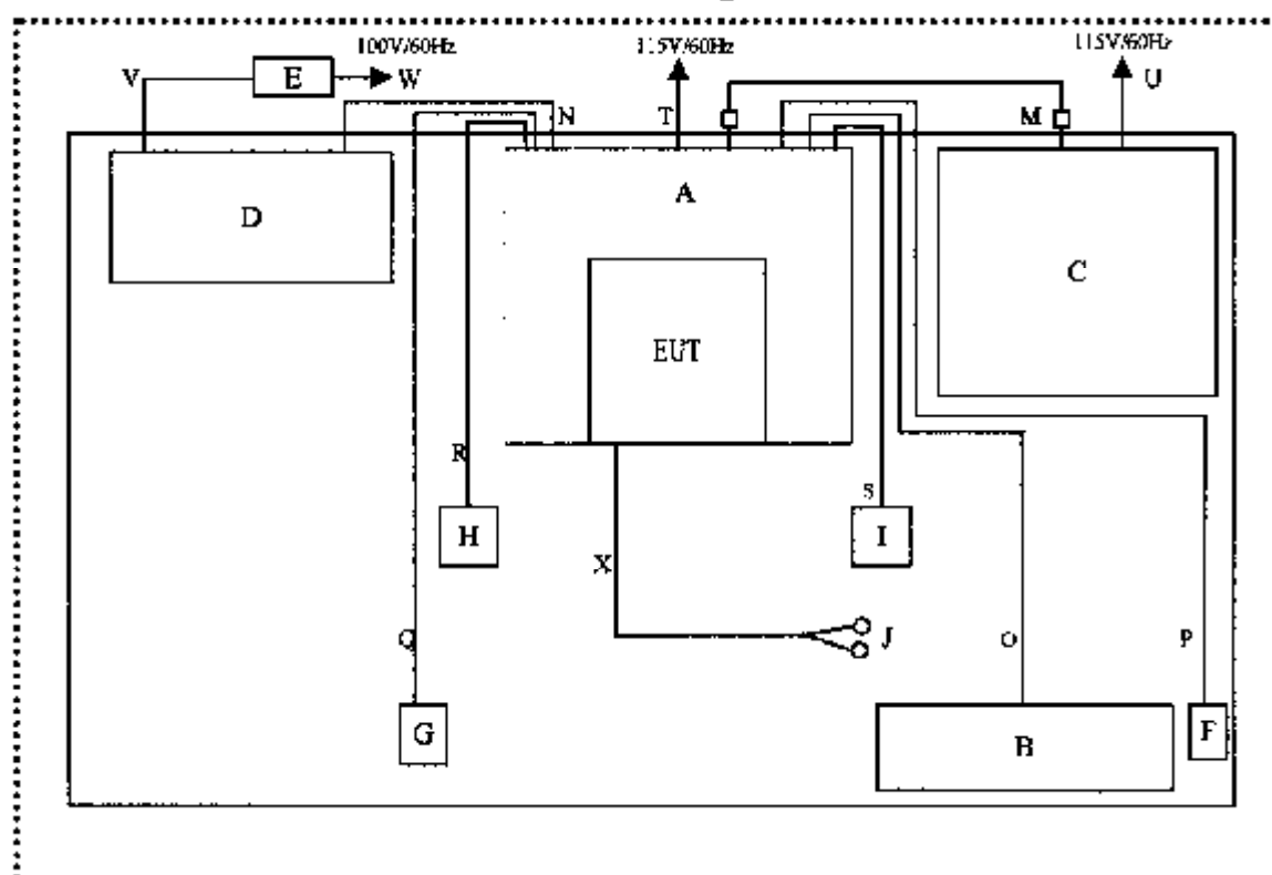
EUT's Test Arrangement
