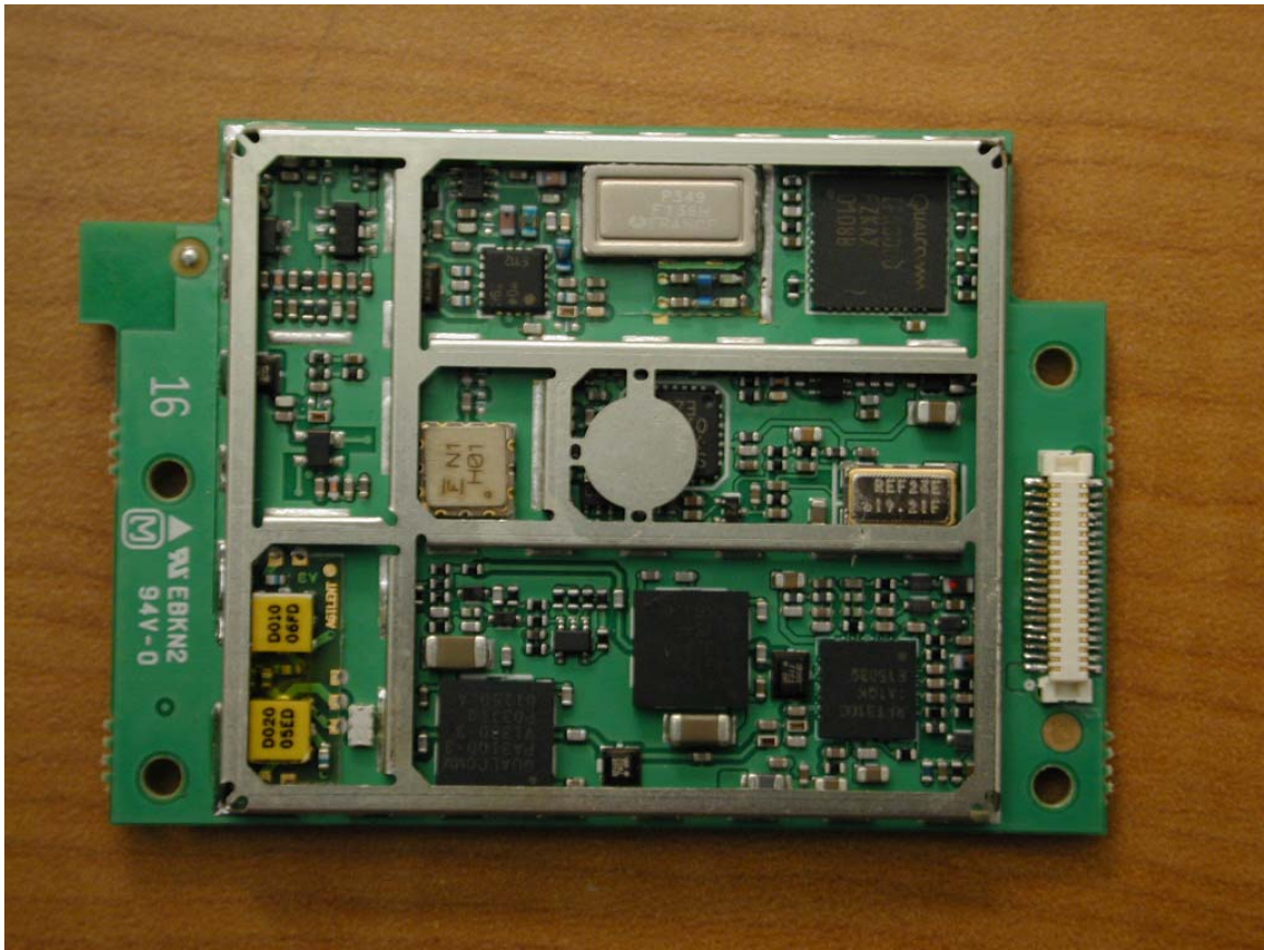
RF Components with Shield Fence
