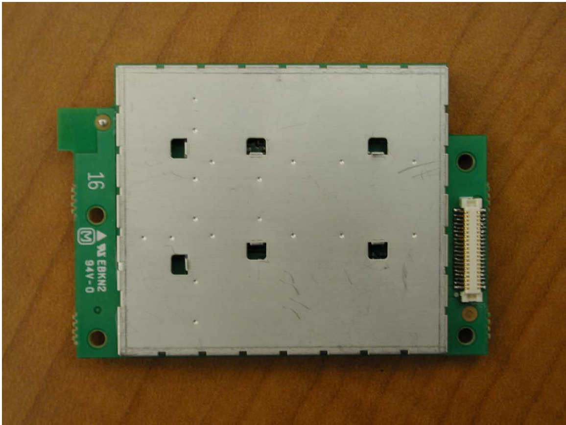
RF Side with Shield Cover
