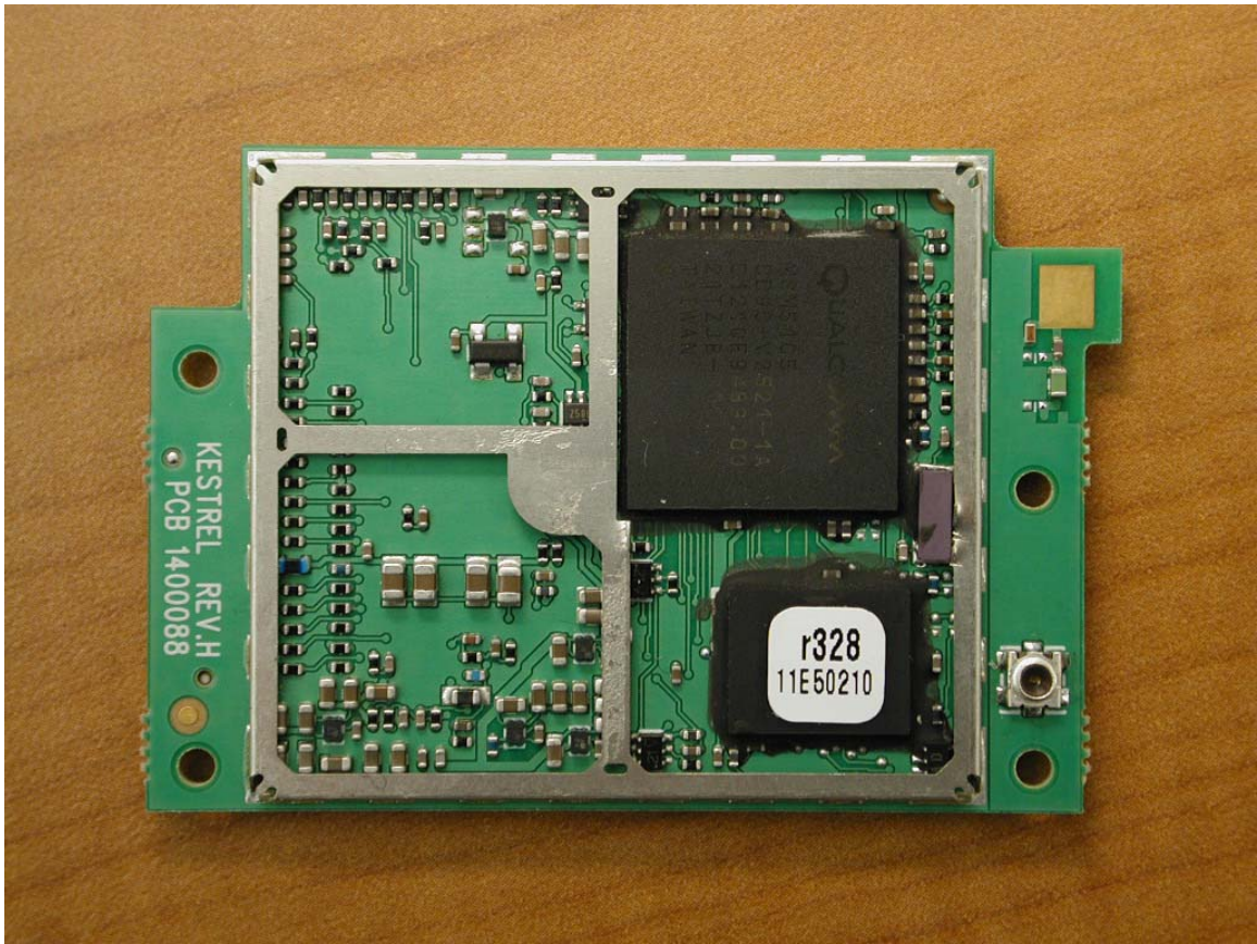
Logic Components with Shield Fence
