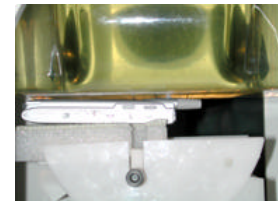
Fig. 18 Hand SAR Test Setup
