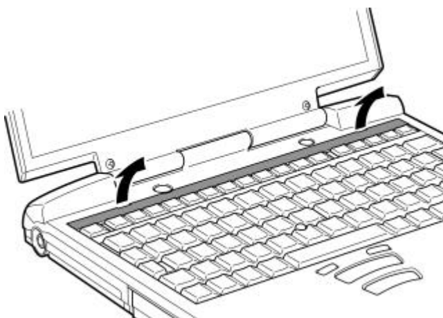
Figure 2 Removing the keyboard brace
