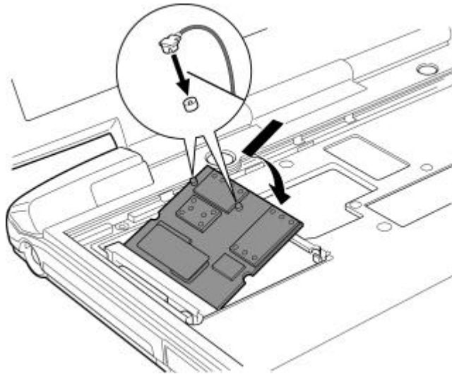
Figure 5 Inserting the Wireless LAN board
