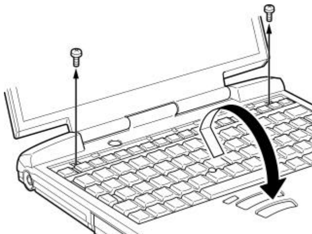
Figure 3 Removing the keyboard
