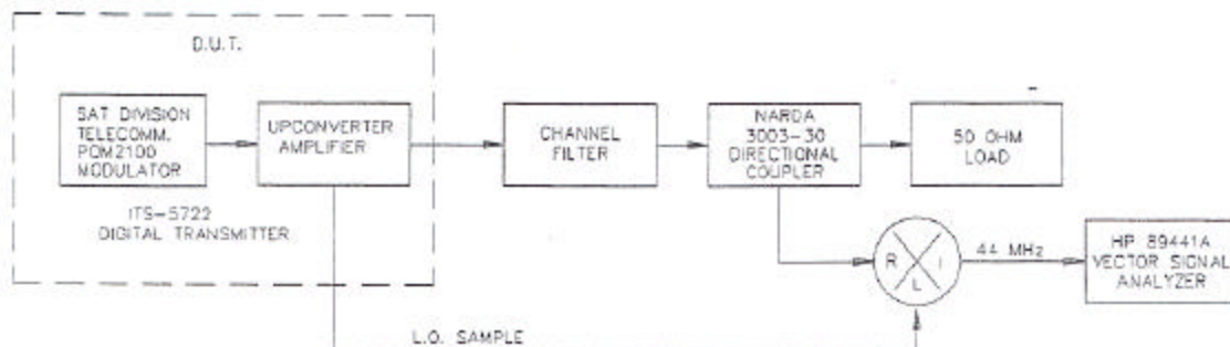
Typical QAM Demodulation Test Set-up
