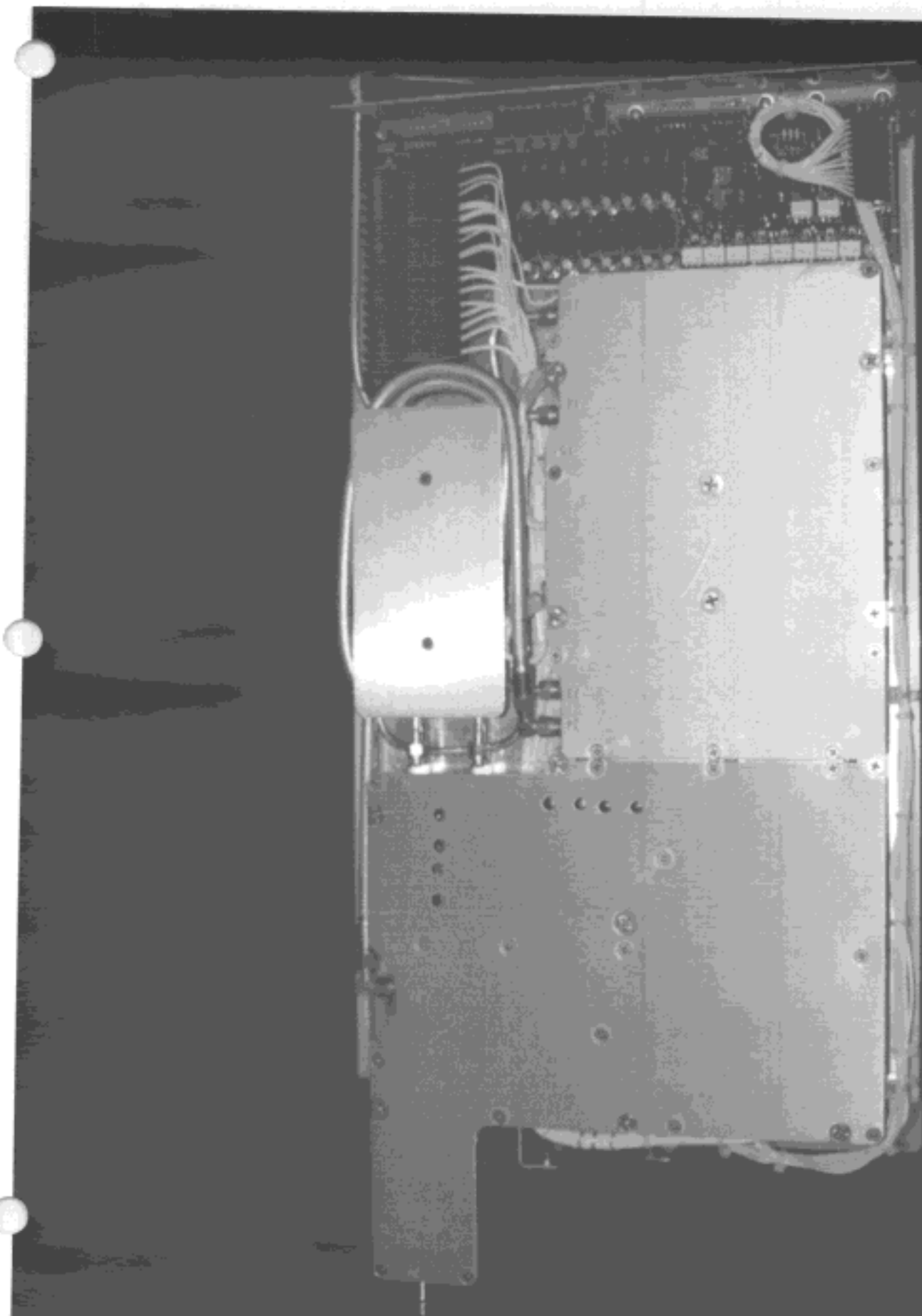
4.3.7 Top view, Broadband Amplifier Tray (25W Amplifier Module)
