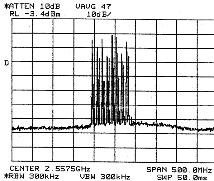
Out-of-Band Power Plot/500 MHz Span (31.5 Watts total average):
