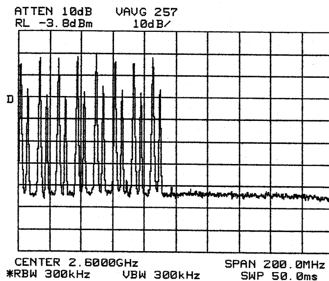
Occupied Bandwidth Plot/200 MHz Span (63.0 Watts total average):
