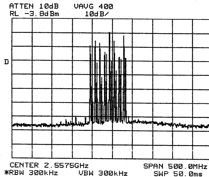
Out-of-Band Power Plot/500 MHz Span (63.0 Watts total average):
