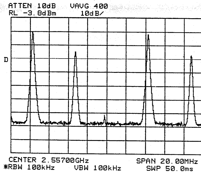
Unoccupied Channel Emissions Plot (63.0 Watts total average):
