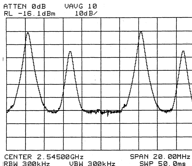
Unoccupied Channel Emissions Plot (1.0 Watts total average):
