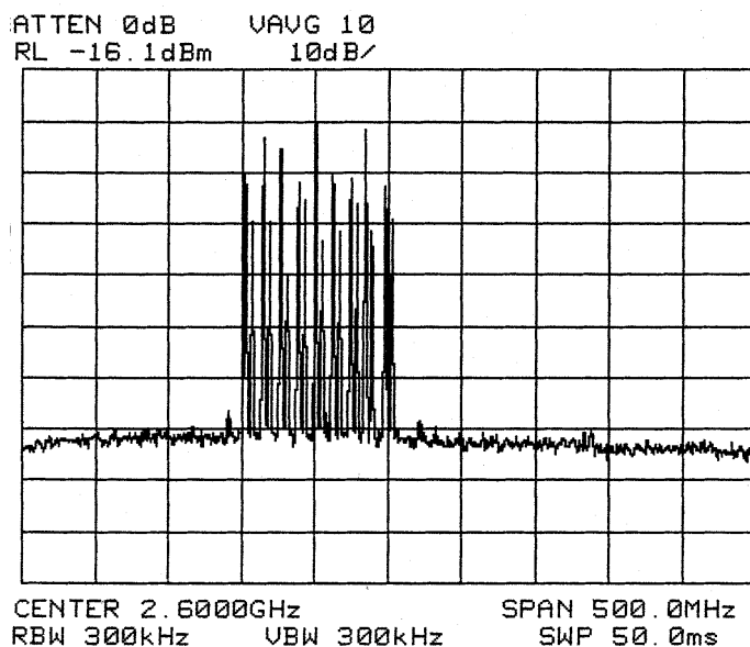
Out-of-Band Power Plot/500 MHz Span (1.0 Watts total average):
