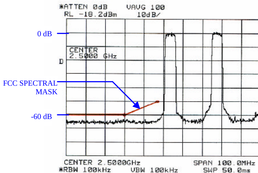
Figure 3.3.1 Spectrum Analyzer Plot (Showing Lower Band Edge) With Four Channels Present (A1, A3, G2 and G4)
