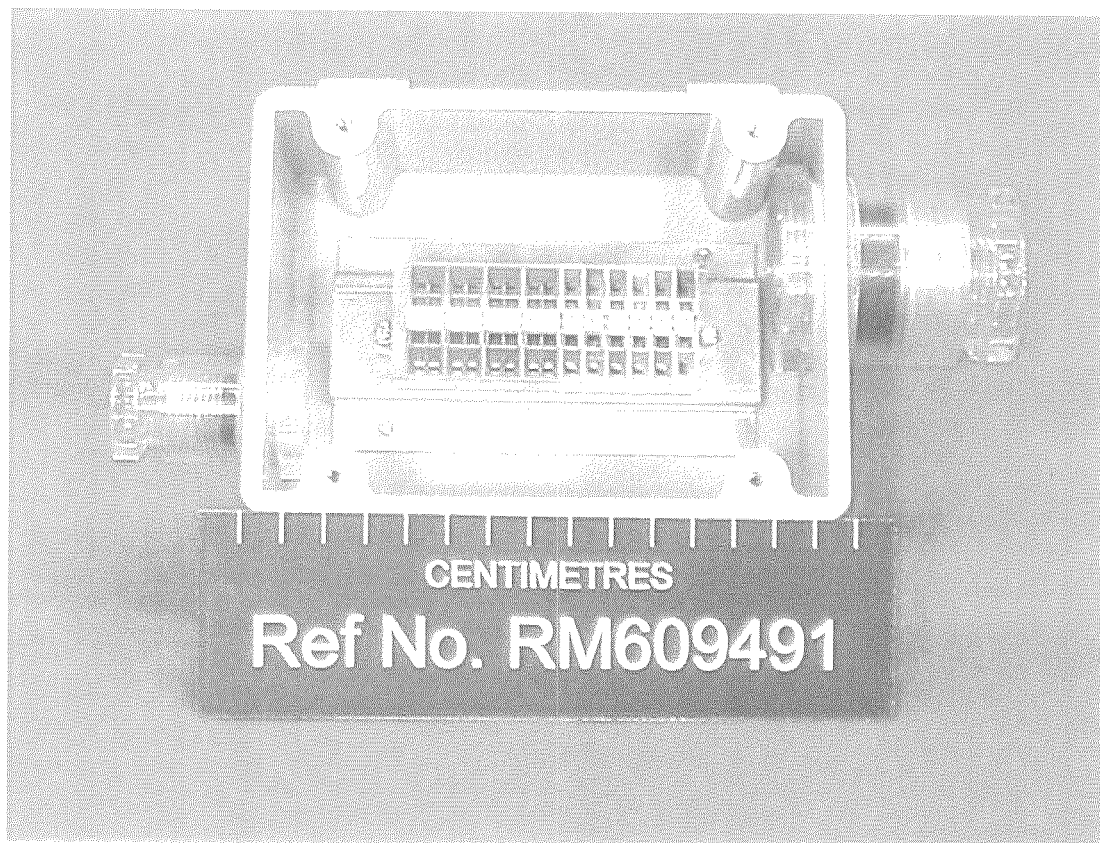
NQD-4190 Junction Box – Internal View
