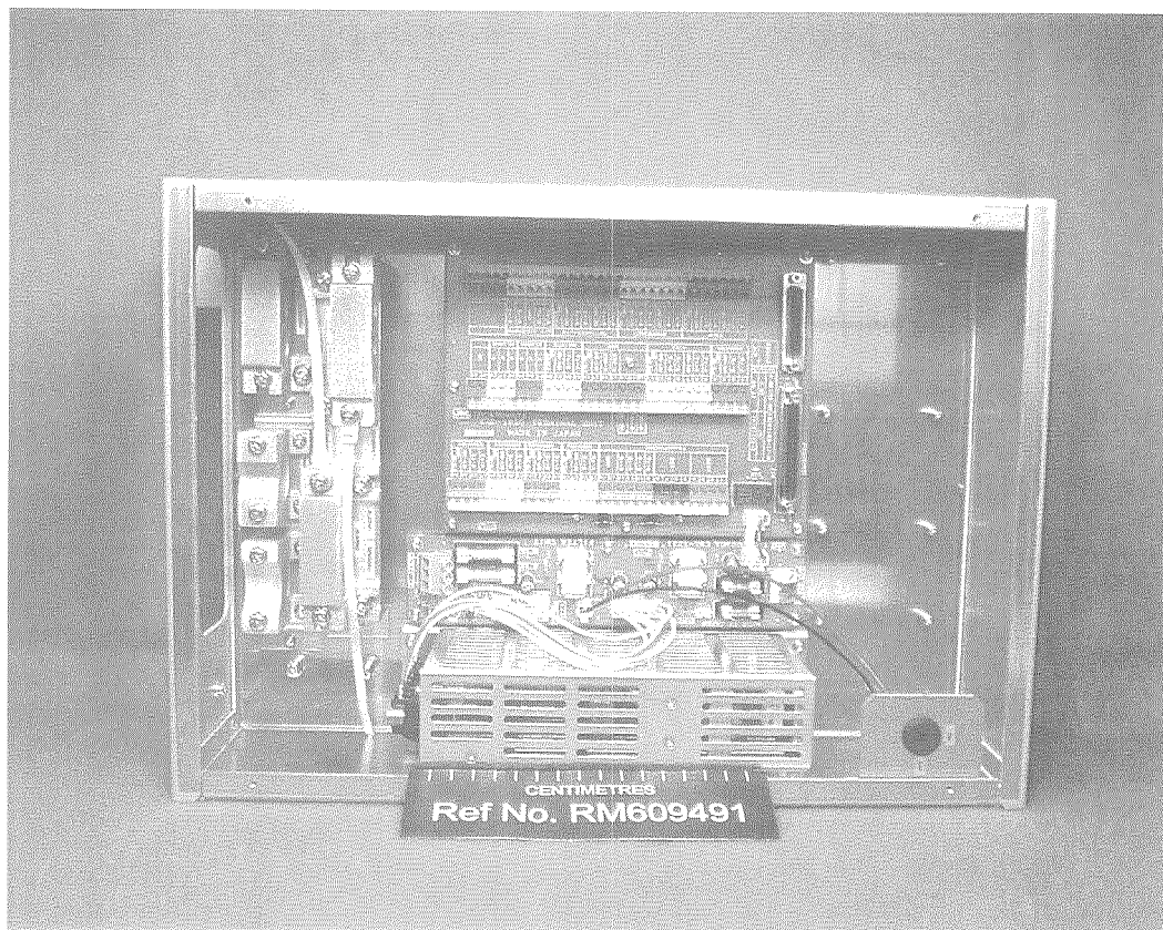
NQE-3111 Connection Box – Internal View
