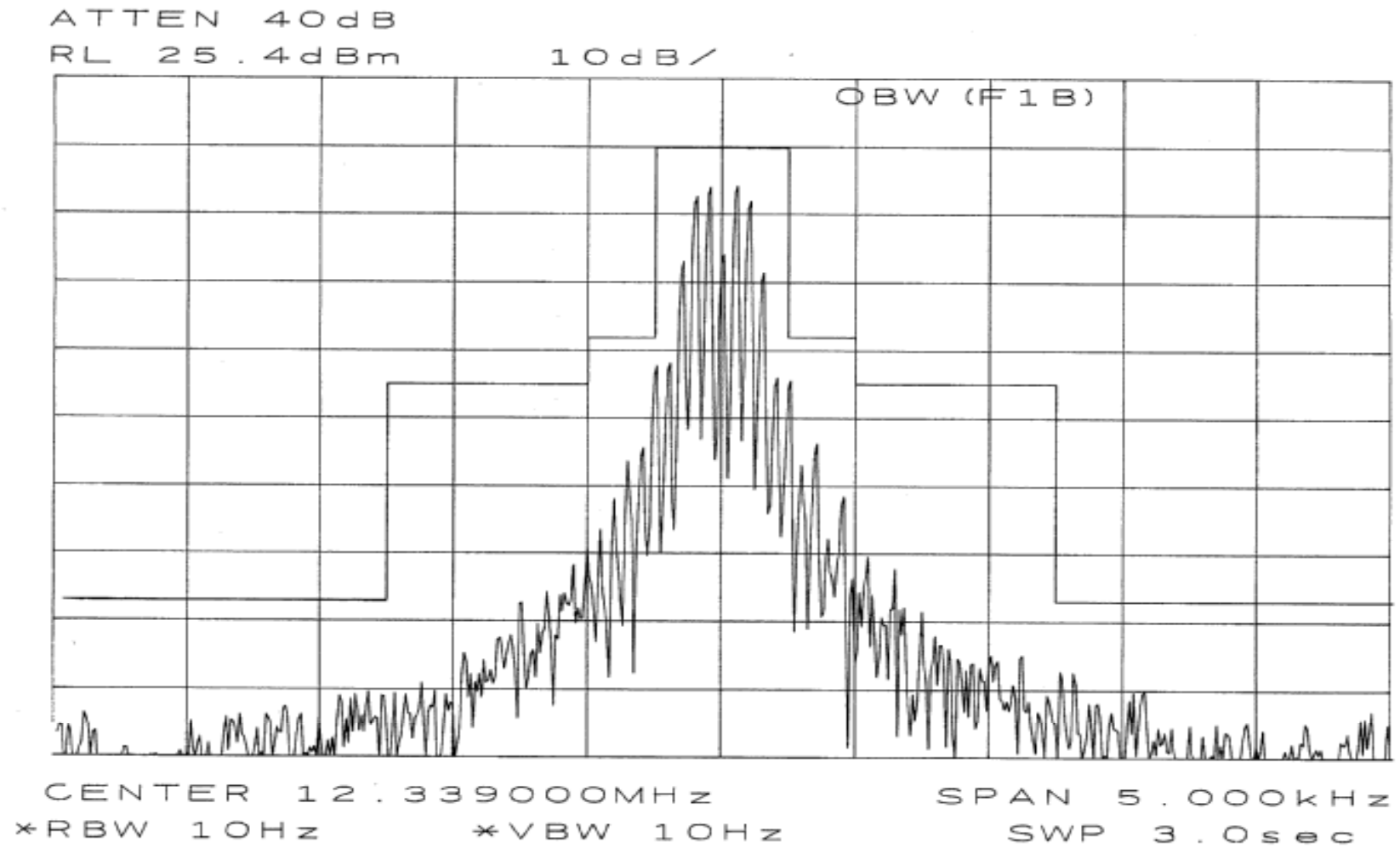
Fig. 2.3.2-27 Occupied bandwidth
