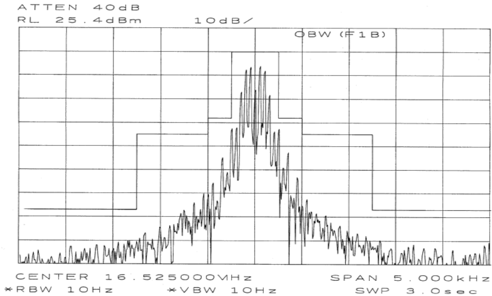
Fig. 2.3.2-30 Occupied bandwidth
