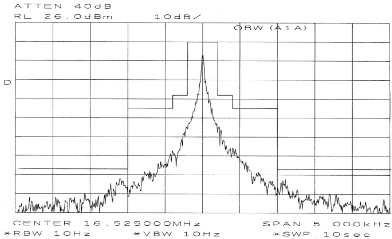
Fig. 2.3.2-29 Occupied bandwidth
