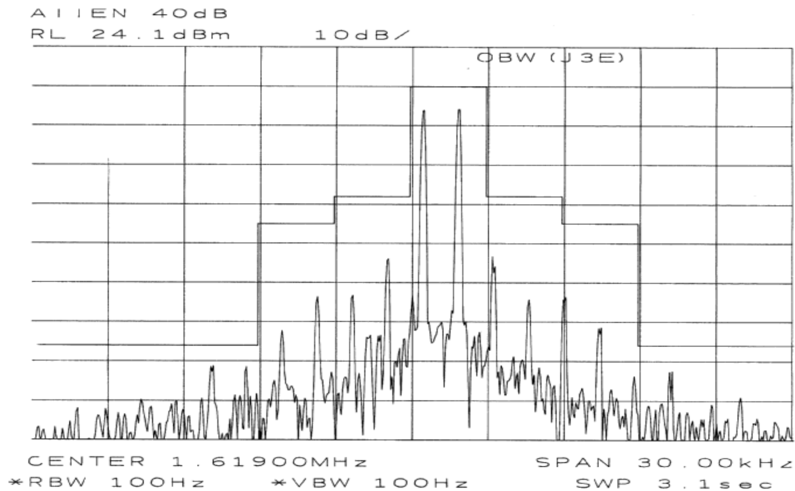
Fig. 2.3.2-1 Occupied bandwidth
