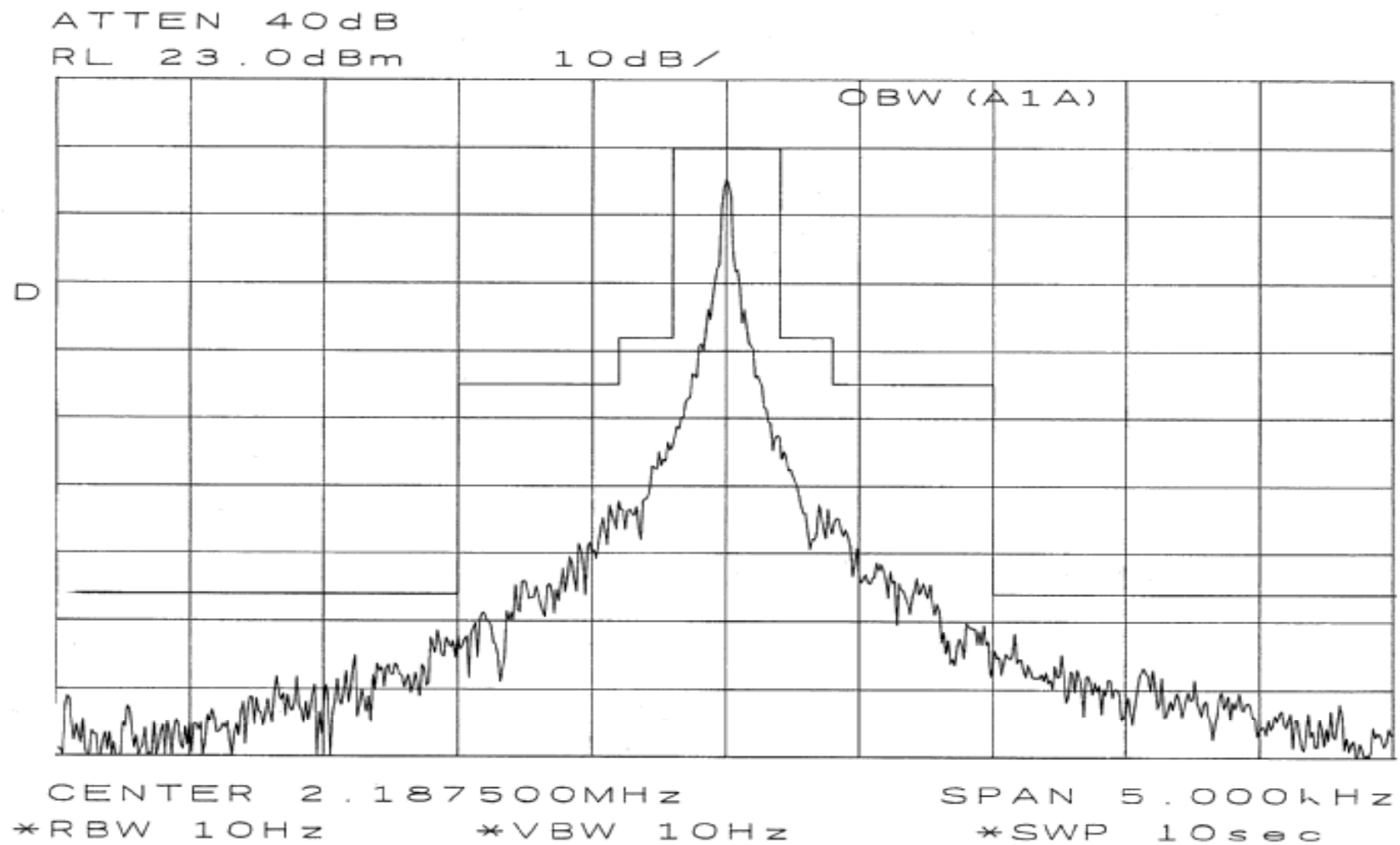
Fig. 2.3.2-8 Occupied bandwidth
