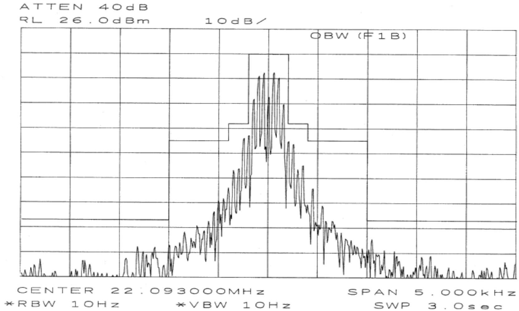
Fig. 2.3.2-33 Occupied bandwidth
