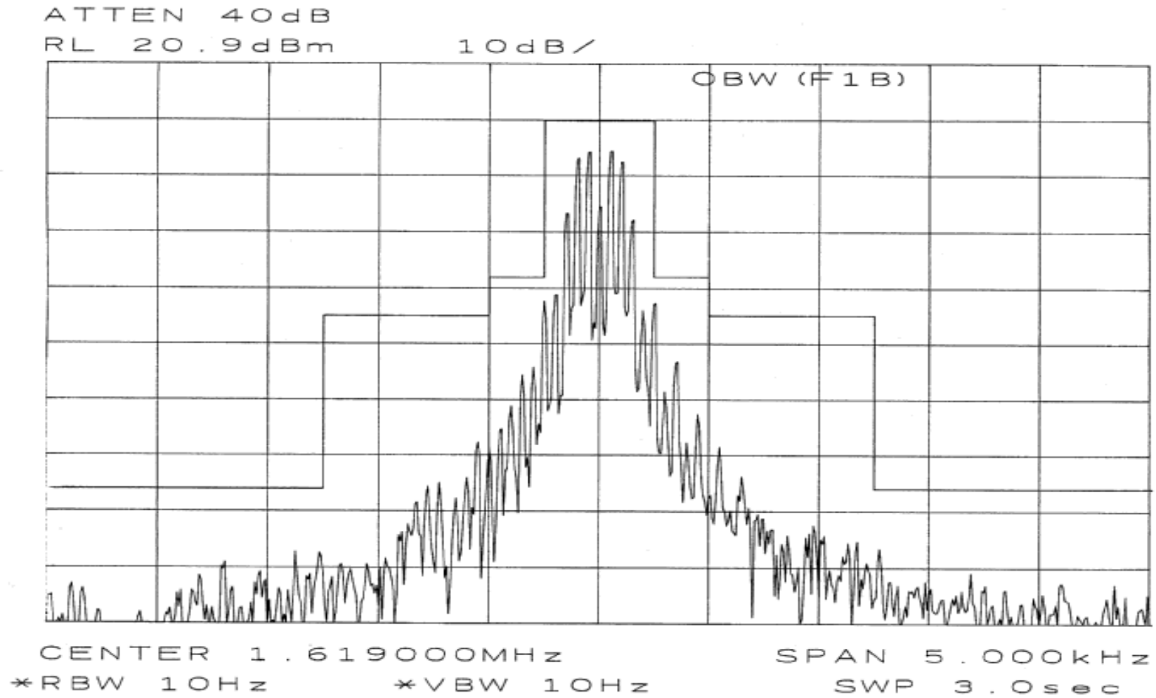
Fig. 2.3.2-3 Occupied bandwidth
