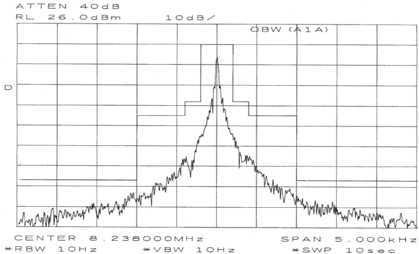
Fig. 2.3.2-23 Occupied bandwidth
