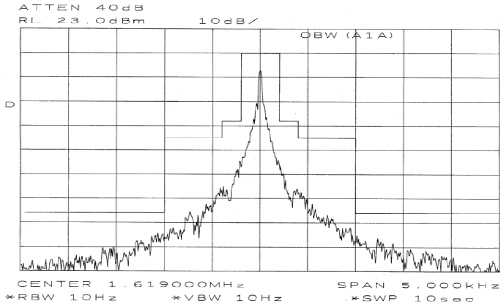
Fig. 2.3.2-2 Occupied bandwidth
