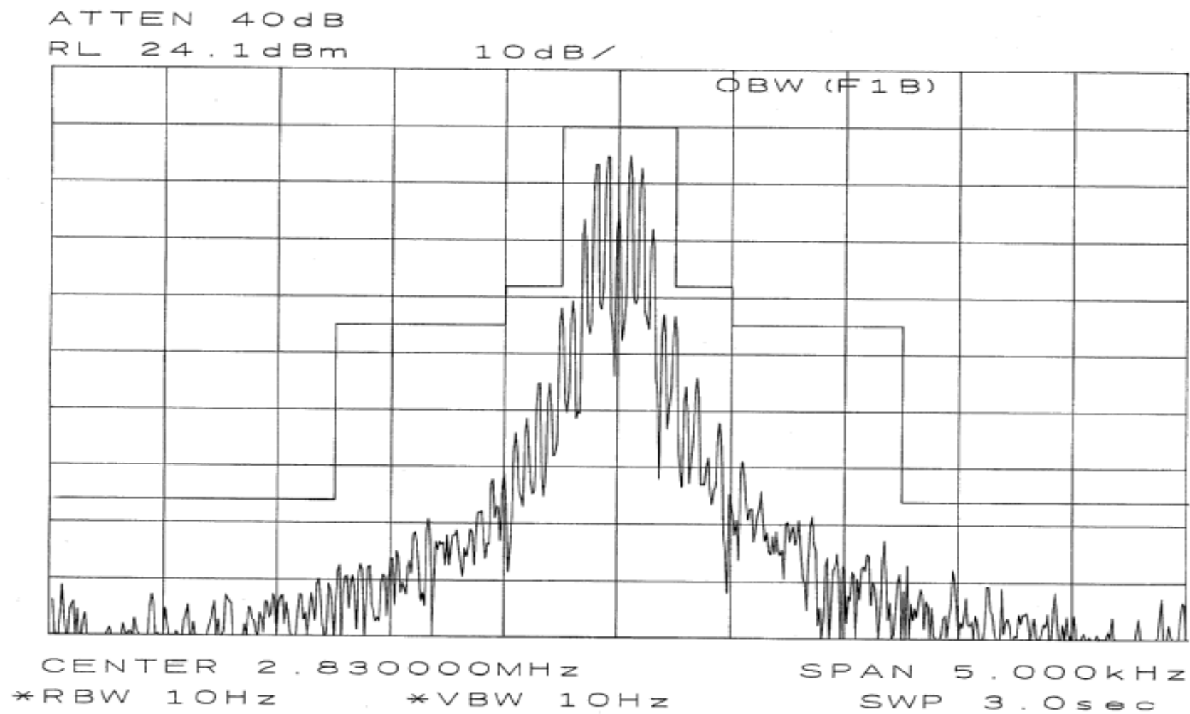
Fig. 2.3.2-12 Occupied bandwidth
