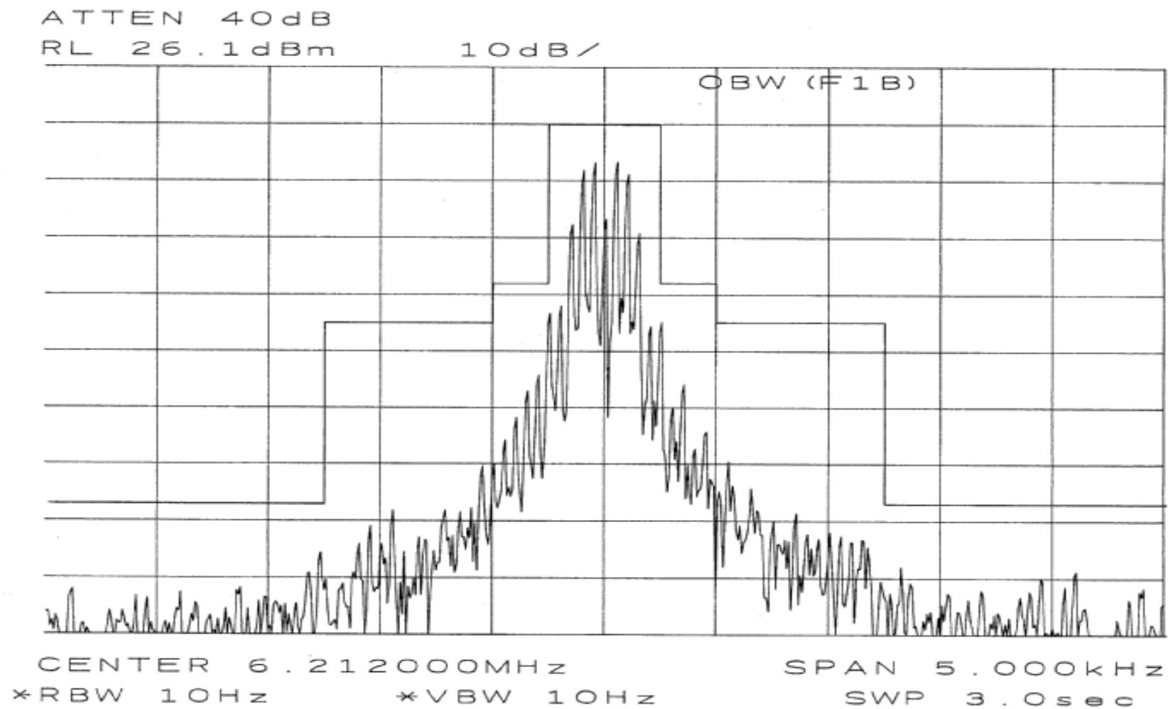
Fig. 2.3.2-21 Occupied bandwidth
