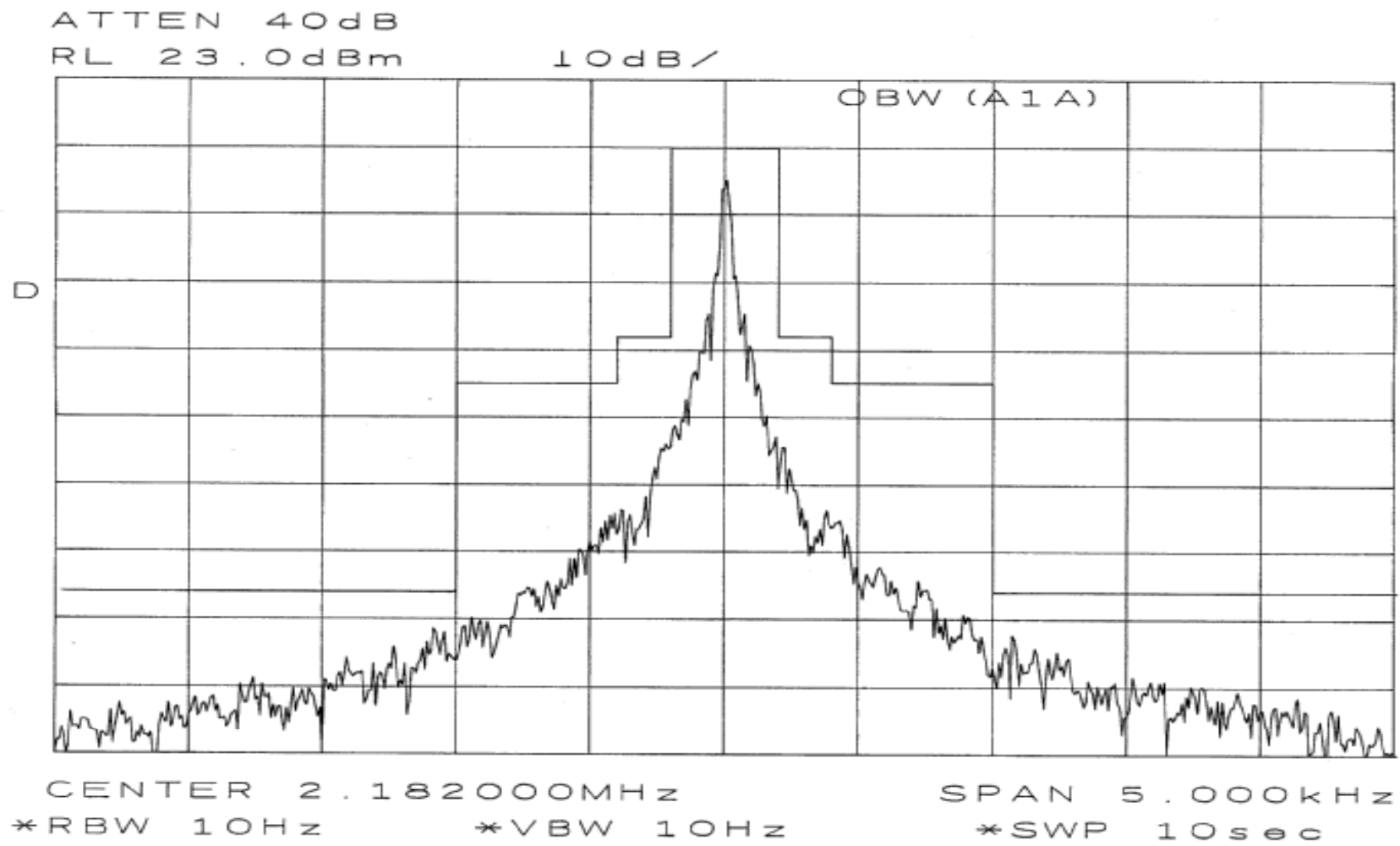
Fig. 2.3.2-5 Occupied bandwidth
