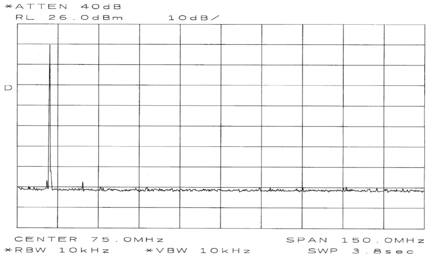
Fig. 2.4.2-9 Spurious emissions at antenna terminal
