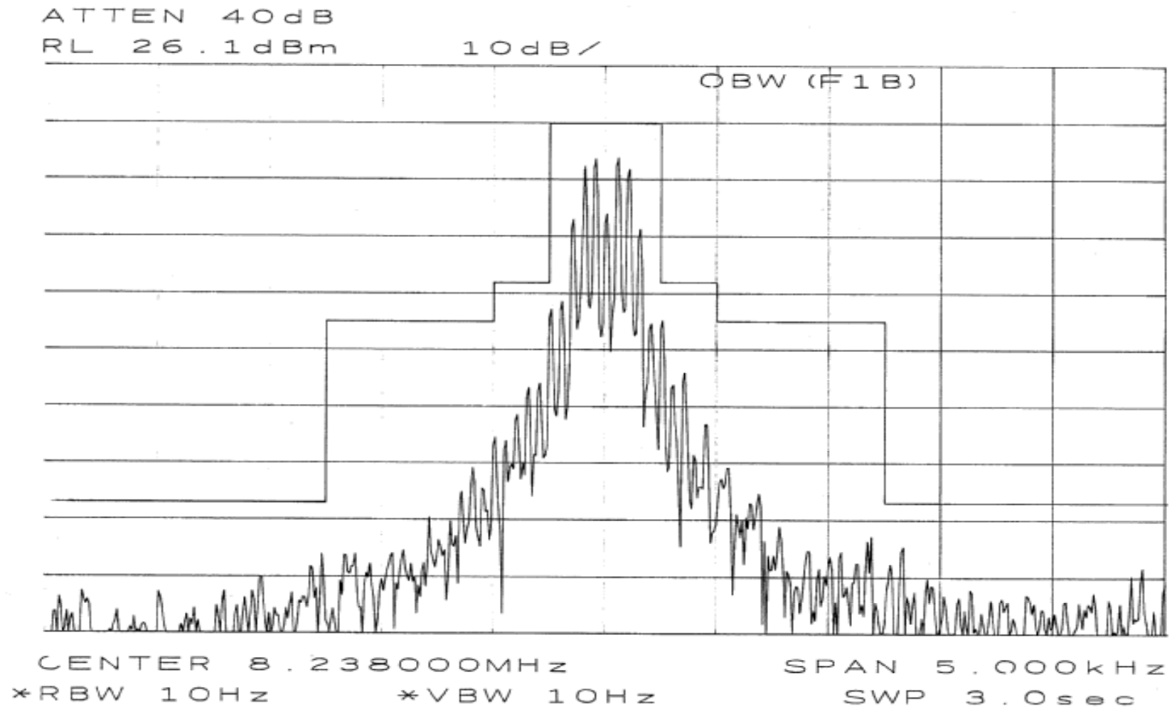
Fig. 2.3.2-24 Occupied bandwidth
