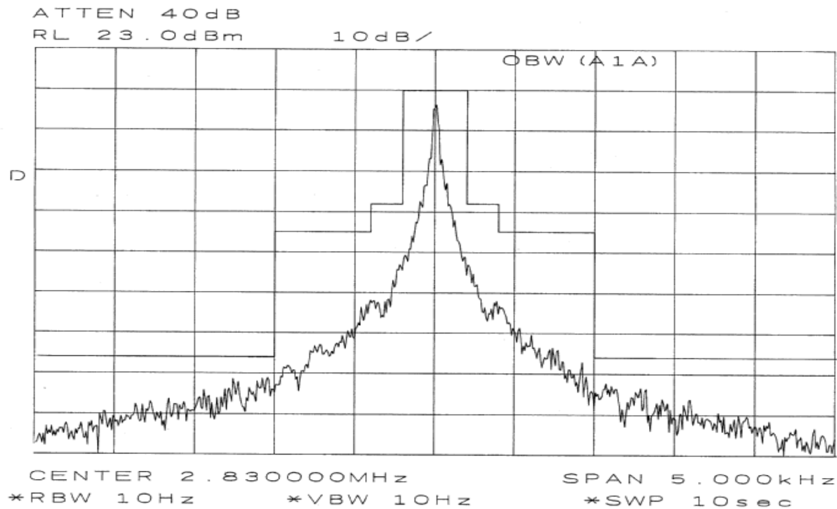
Fig. 2.3.2-11 Occupied bandwidth
