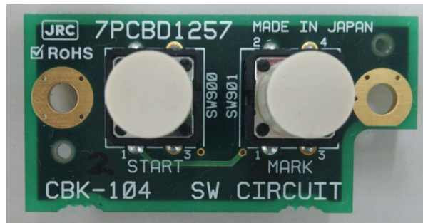
Parts side
