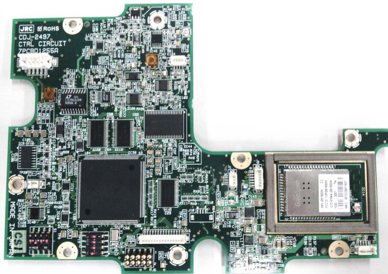
Parts side
