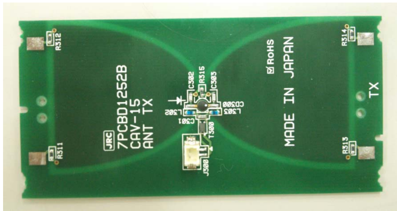
Parts side
