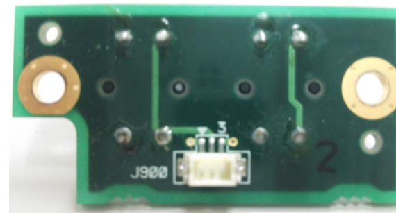
Solder side
