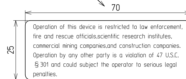
Detail view (1:1)
