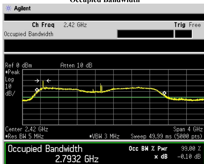
Occupied Bandwidth
