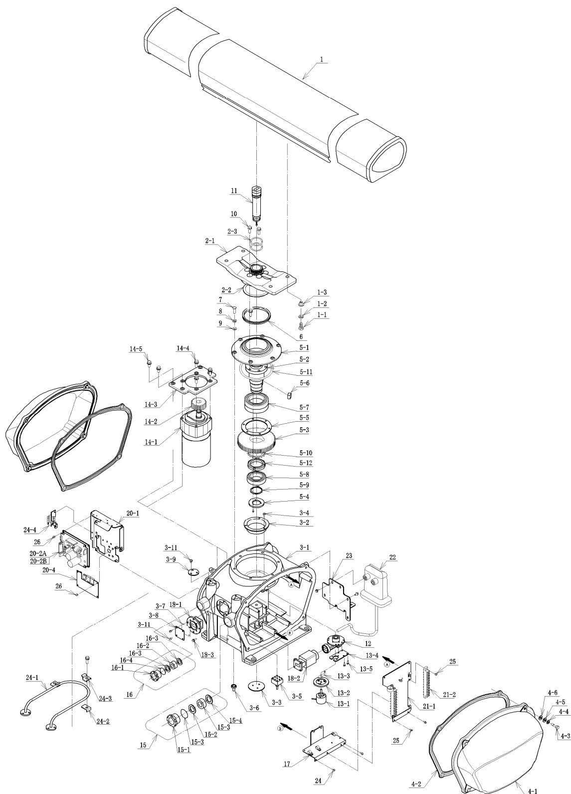
NKE-1129 SCANNER UNIT
