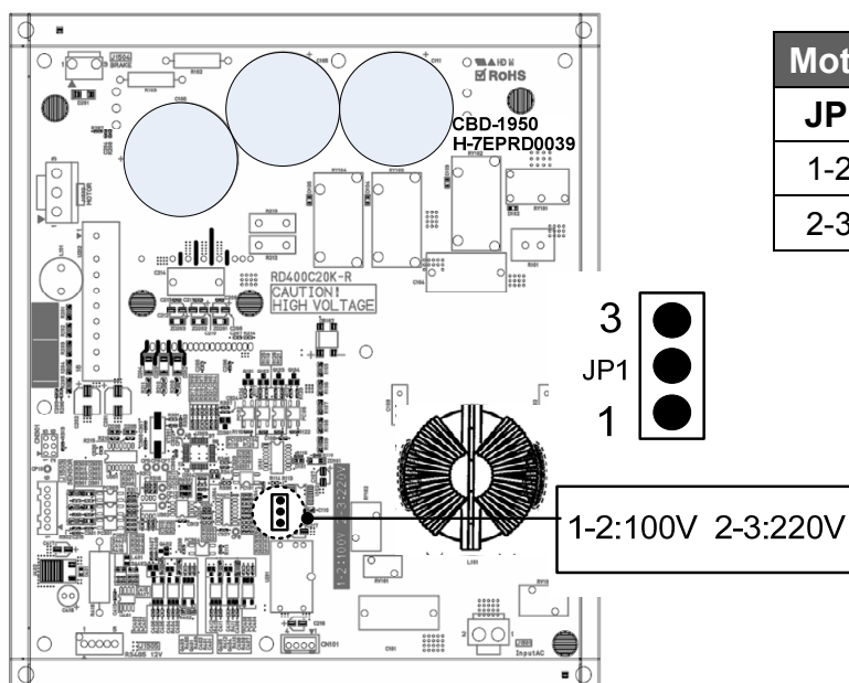
Motor Driver Circuit CBD-1950
