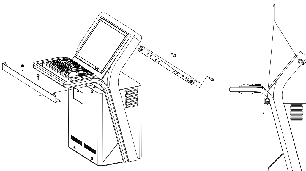
Fig 3-21 When the stand alone type display unit(19inch)
