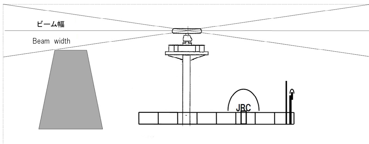
Fig 2-18 Scanner and the surrounding structural objects
