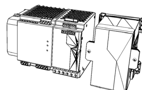
• QUINT-PS/1AC/24DC/20 • QUINT-BAT/24DC/3.4AH • QUINT-DC-UPS/24DC/20 • ME-MAX-NEF/QUINT20 UPS
