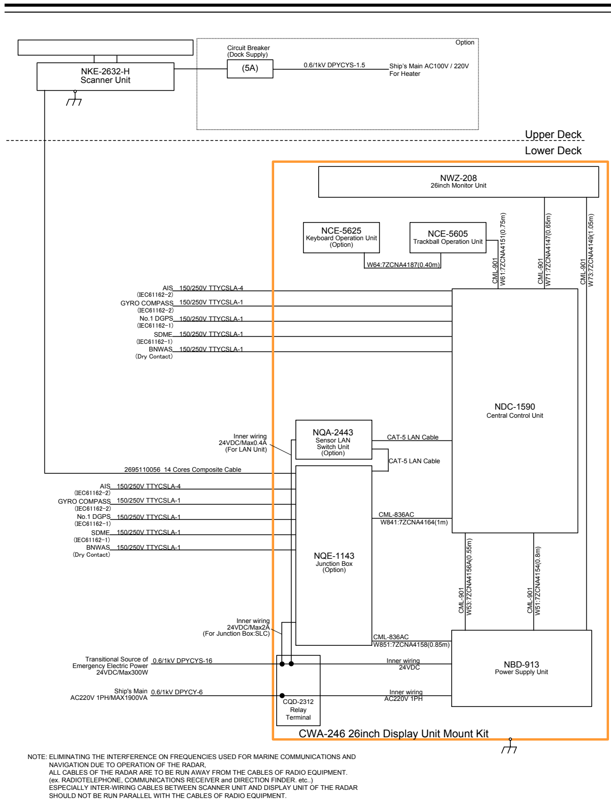
General System Diagram of JMR-9282-SH
