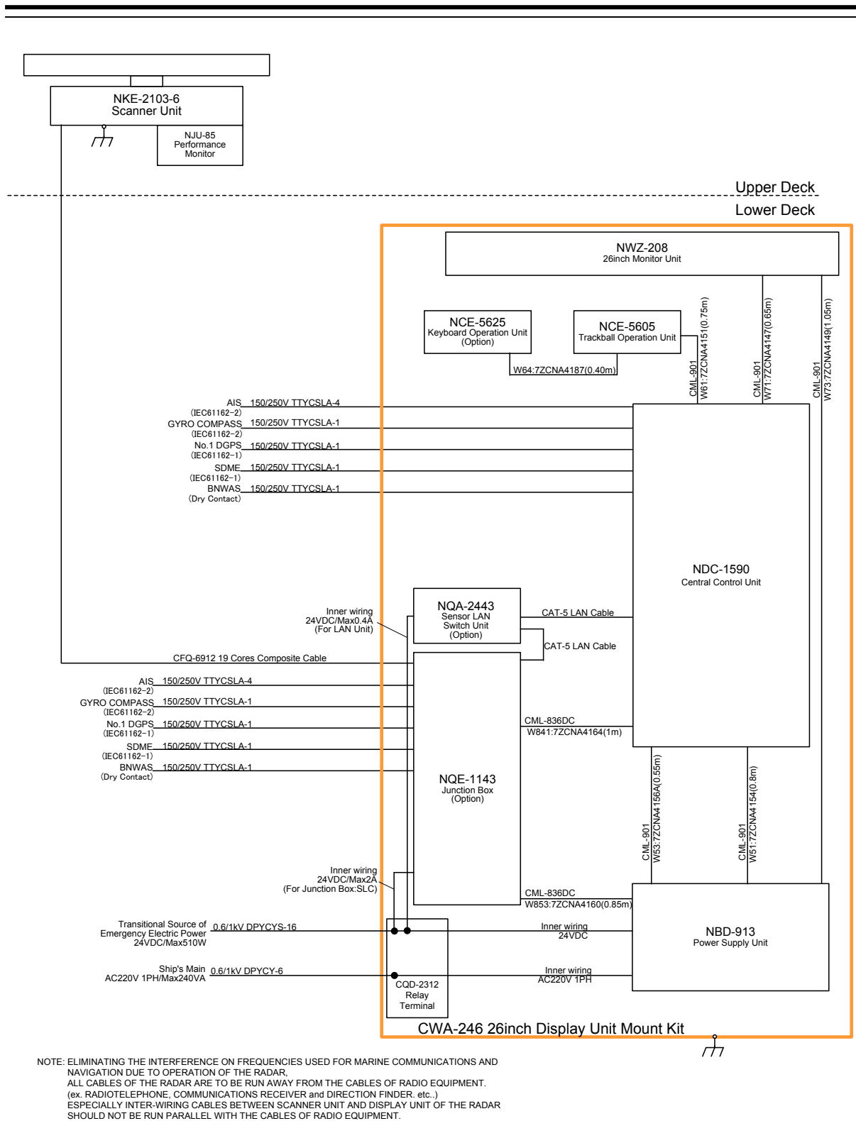
General System Diagram of JMR-9210-6X
