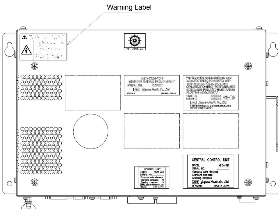
NDC-1590 Central Processing Unit
