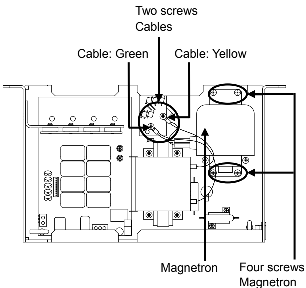
Modulator after the cover is removed
