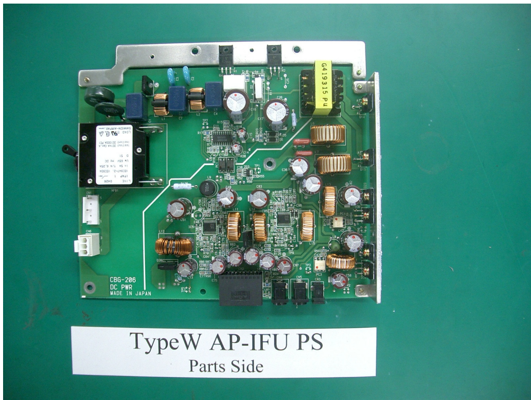
TypeW AP-IFU PS Parts Side Internal View
