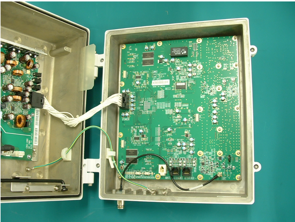
TypeW AP-IFU Internal View 2
