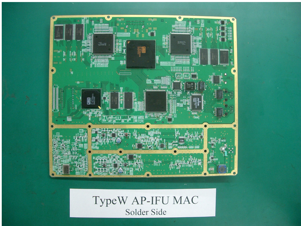
TypeW AP-IFU MAC Solder Side Internal View
