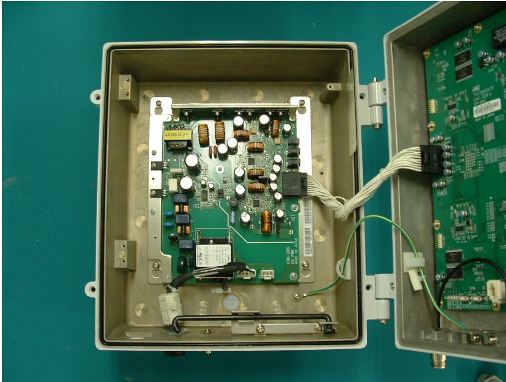
TypeW AP-IFU Internal View 1
