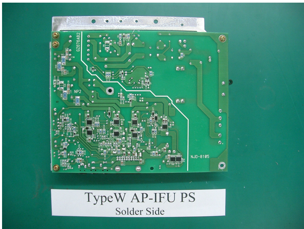
TypeW AP-IFU PS Solder Side Internal View
