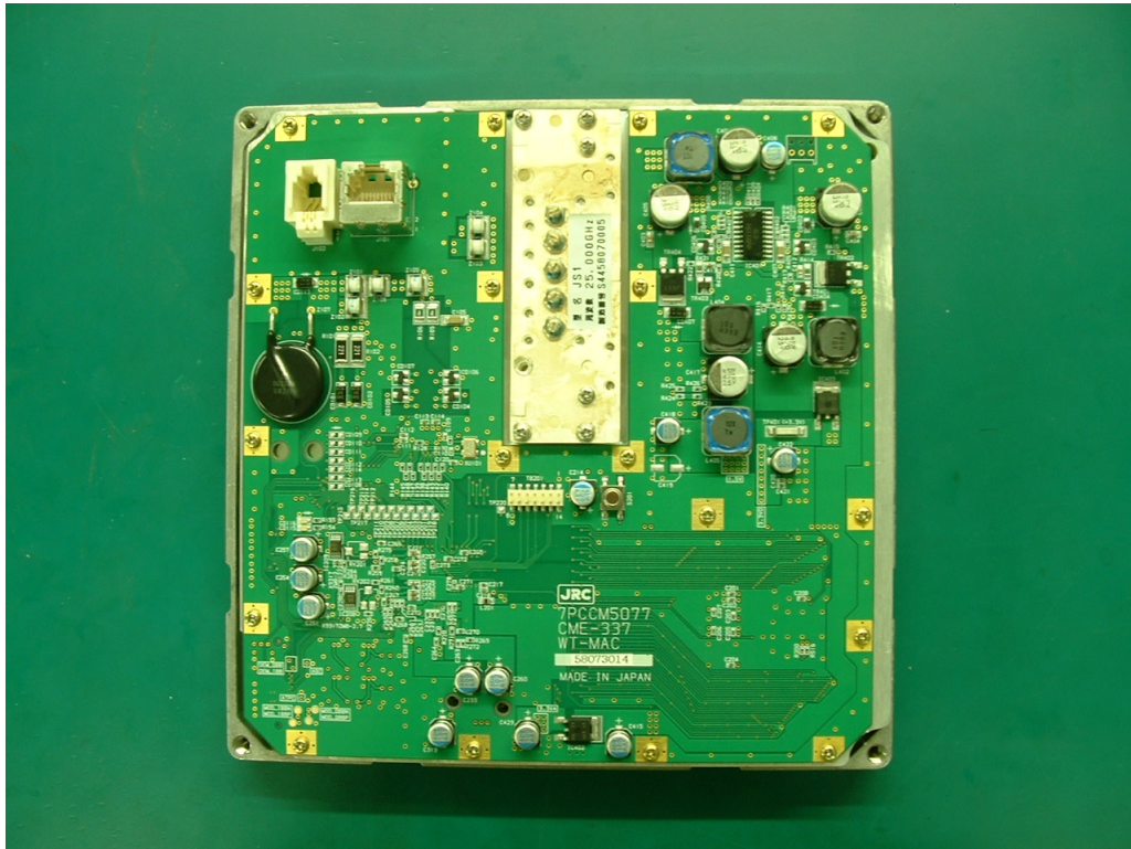
TypeW WT Internal View
