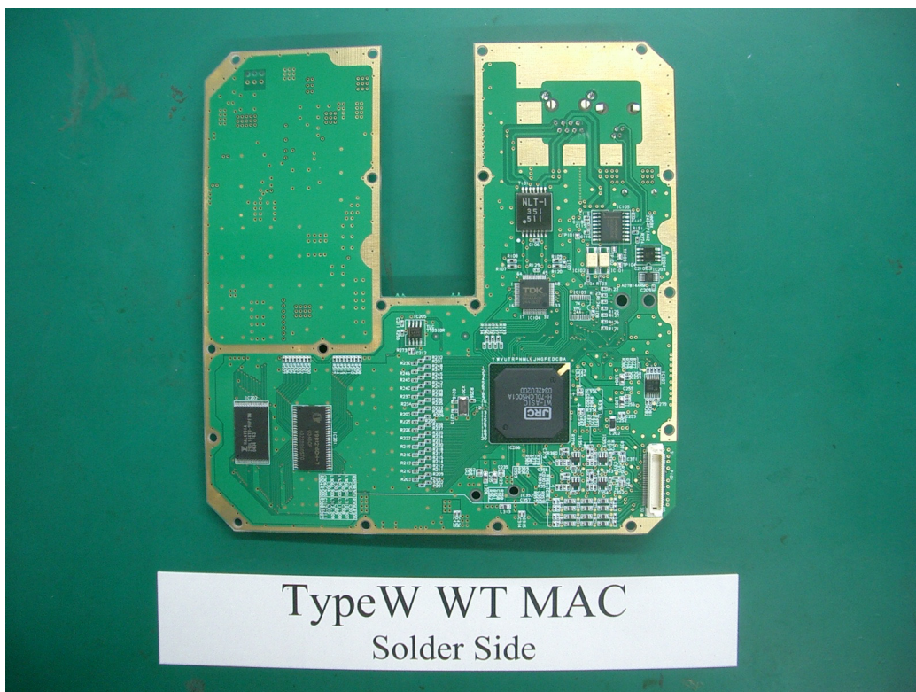
TypeW WT MAC Solder Side Internal View
