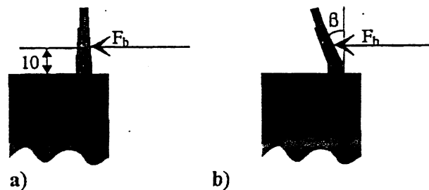
Figure 4.2.1 Helix bending test a) F_b application b) F_b and \beta
