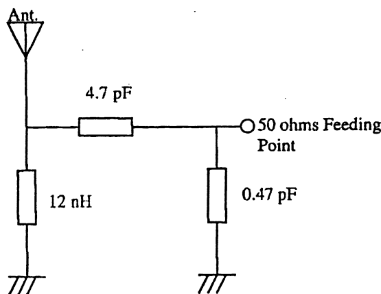
Figure 3.3.1 Matching circuit
