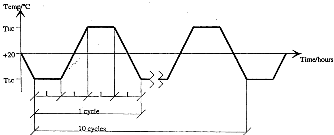
Figure 5.2.1 Temperature cycling
