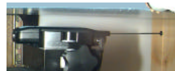
Figure 16. Body SAR Test Setup
