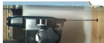
Figure 16. Body SAR Test Setup
