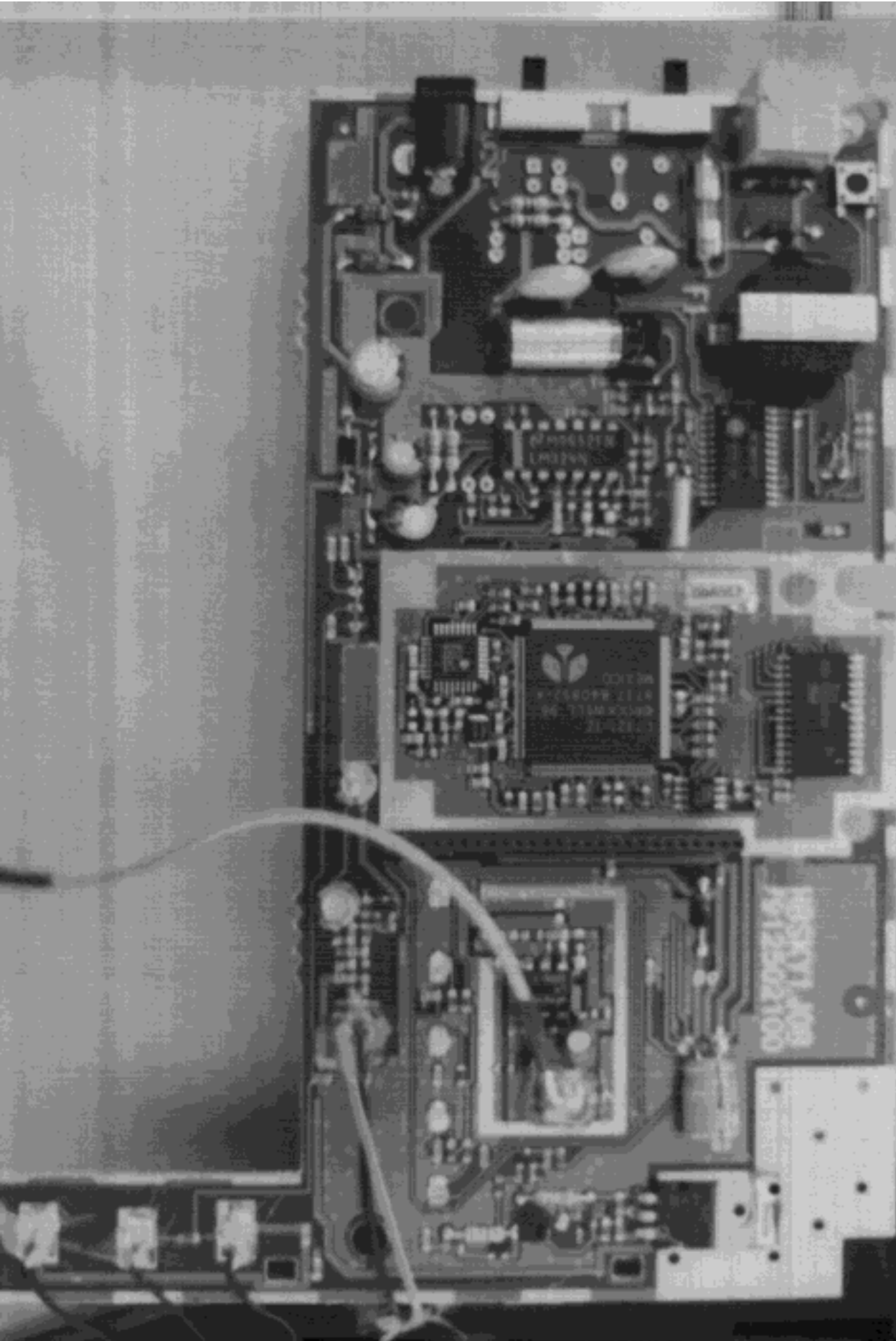
TOP VIEW OF MAIN BOARD OF BASE FCC ID: CLH5KYHAWK98
