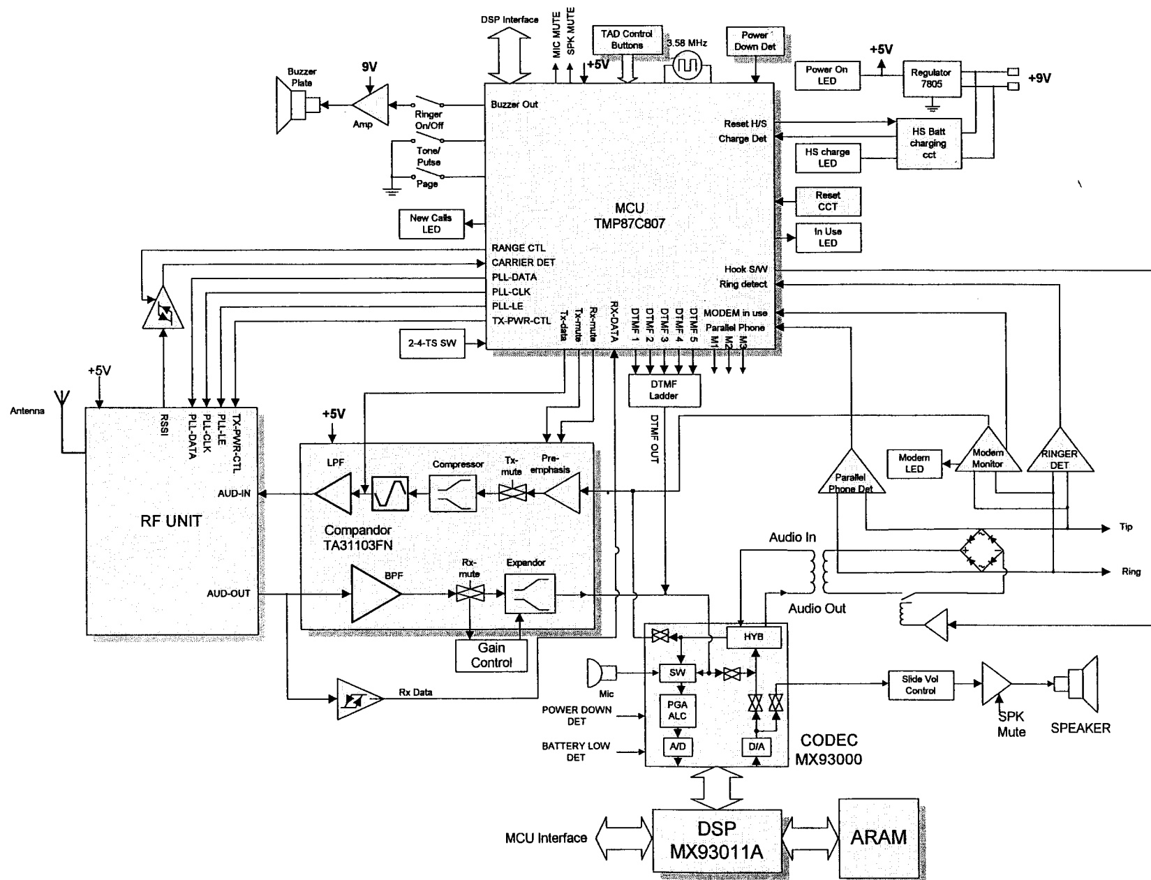
TC-920 Base Block Diagram
