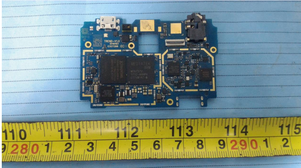
EUT – Mainboard Bottom 1 Shielding off View
